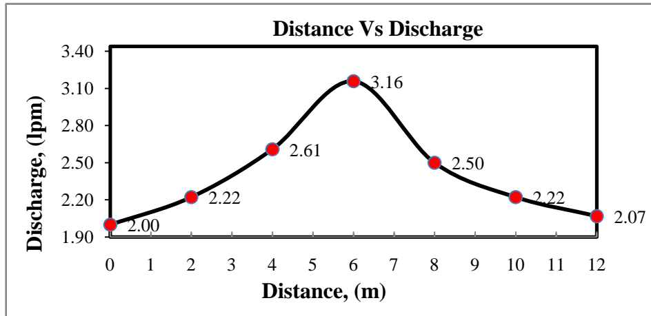
Fig. 3: Relationship between discharge and varying horizontal carrying distance at constant suction lift (1.22m)
