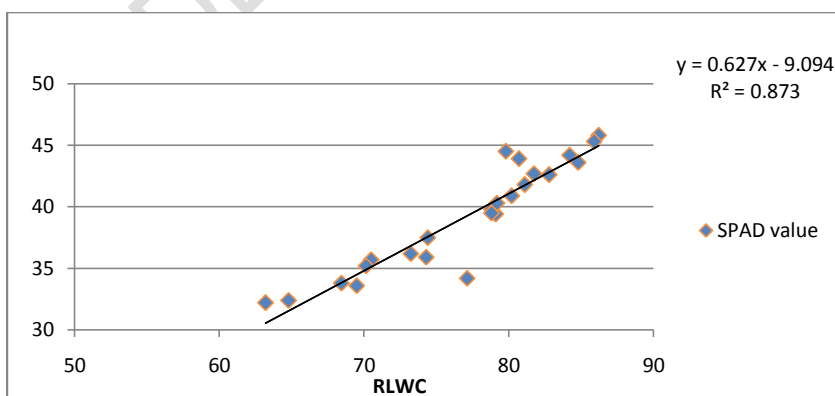
Fig.1. Relationship between RLWC and SPAD values in the year 2022
