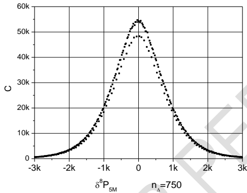
Fig. 18 Scatter-plots of \delta^8 P_{5M} n_{\Delta}=750
