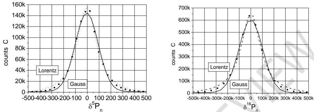
Fig. 2 Scatter-plot & fits for \delta^5 P_{1M} n_{\Delta}=50 Fig. 3 Scatter-plots & fits for \delta^{16} P_{3M} n_{\Delta}=50
