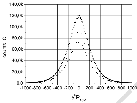
Fig. 22 Scatter-plots of \delta^6 P_{10M} n_{\Delta}=800 Fig. 23 Scatter-plots of \delta^6 P_{10M} n_{\Delta}=1,200
