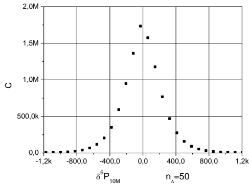
Fig. 20 Scatter-plot of \delta^6 P_{10M} n_{\Delta}=50 Fig.21 Scatter-plots of \delta^6 P_{10M} n_{\Delta}=400
