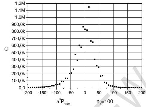
Fig. 27 Scatter-plot(s) of \delta^3 P_{10M} n_{\Delta}=100
