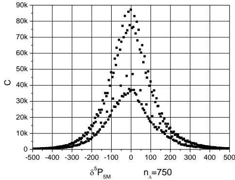
Fig. 12 Scatter-plots of \delta^5 P_{5M} n_{\Delta}=750
