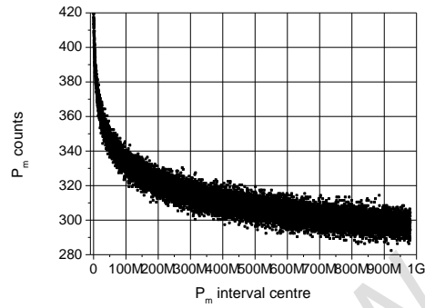
Fig. 43 Scatter-plots of P_{50M} \ 1/8 \ n_{\Delta}=200 Fig. 44 Scatter-plots of P_{50M} \ 1/8 \ n_{\Delta}=20K
