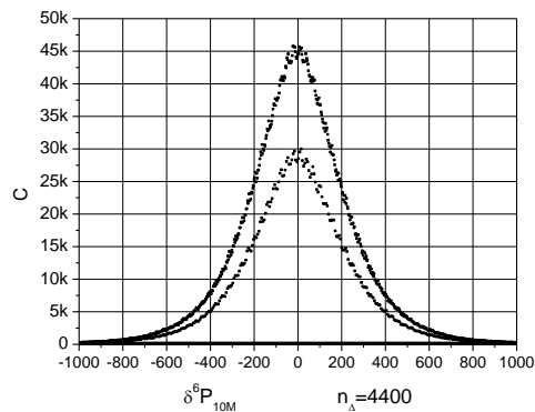
Fig. 24 Scatter-plots of \delta^6 P_{10M} n_{\Delta}=1,600 Fig. 25 Scatter-plots of \delta^6 P_{10M} n_{\Delta}=4,400
