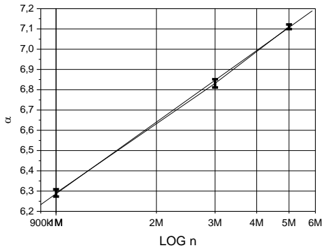
Fig. 7 Coefficient \alpha_0 for Lorentz area vs. n
