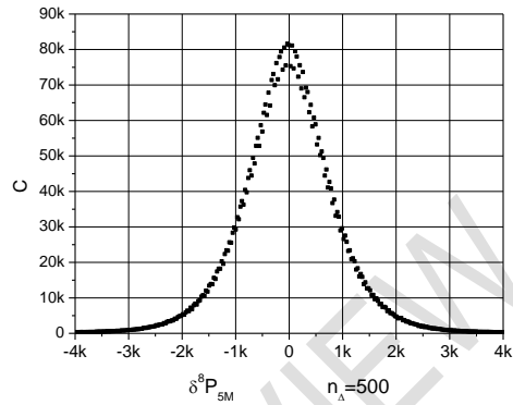
Fig. 16 Scatter-plot & fits of \delta^8 P_{5M} n_{\Delta}=150 Fig. 17 Scatter-plots of \delta^8 P_{5M} n_{\Delta}=500
