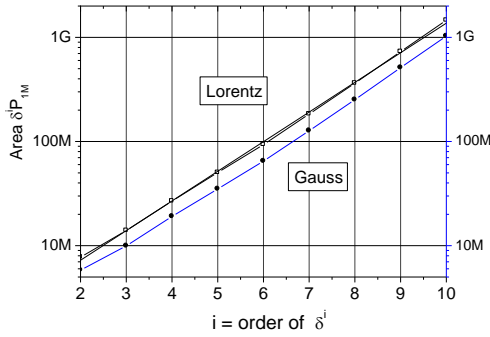
Fig. 4 Areas of the fits vs. order i for 1M
