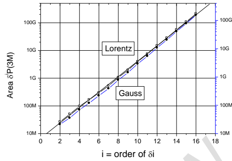
Fig. 5 Areas of the fits vs. order i for 3M
