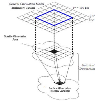
Fig 1. Illustration of Statistical Downscaling
