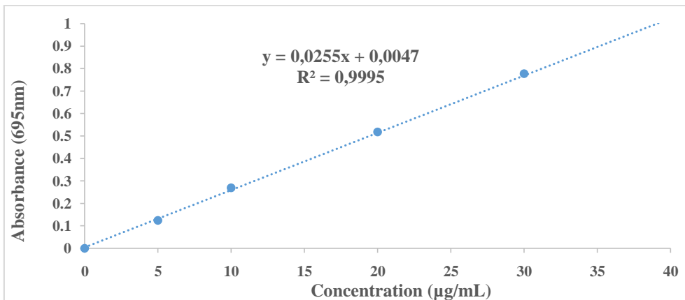
Figure 18 : Calibration curve of Vitamin C
