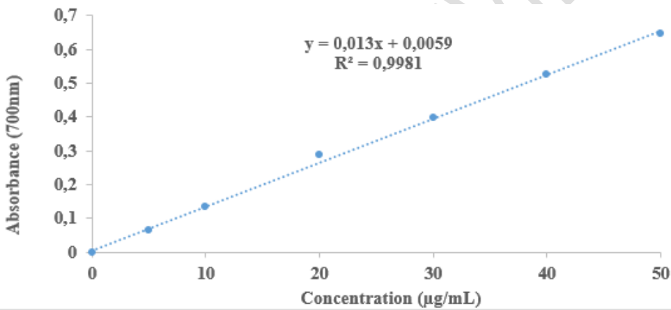
Figure 16 : Calibration curve of vitamin C
