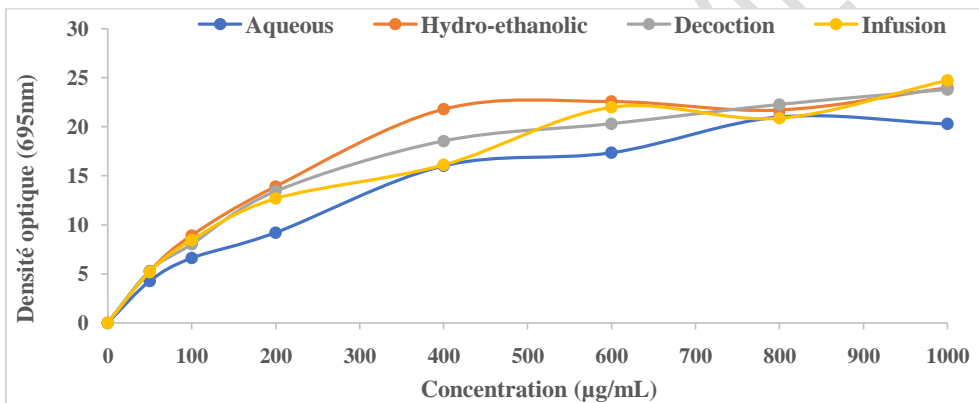
Figure 19 : Phosphomolybdenum test on plant extracts
