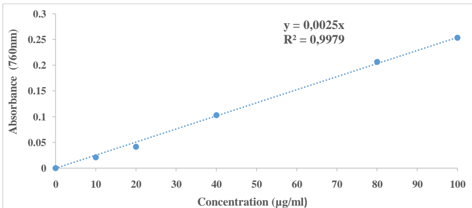
Figure 6 : Calibration of Gallic acid
