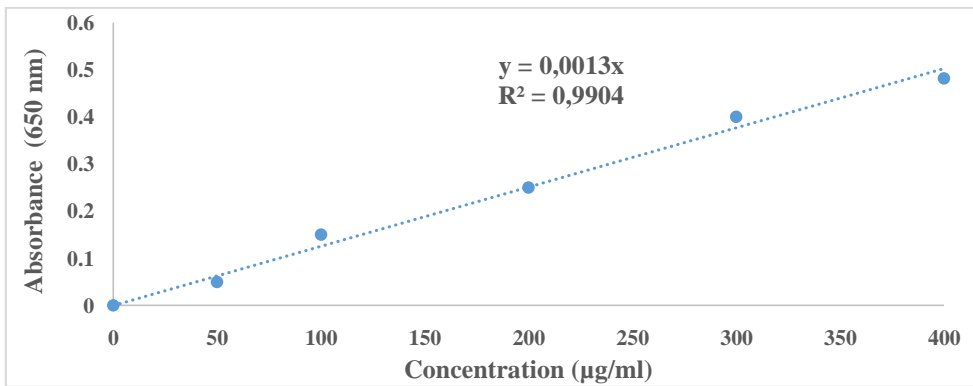
Figure 4 : Calibration curve of bovinalbumine
