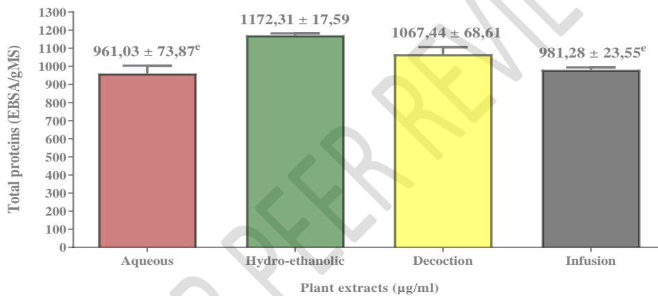
Figure 5 : Concentration of proteins in plant extracts
