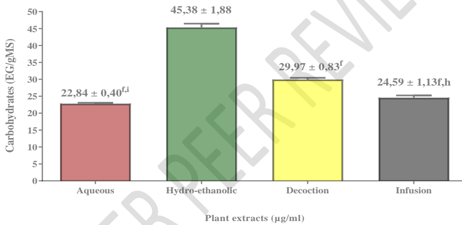
Figure 3 : Concentration of carbohydrates in plant extracts
