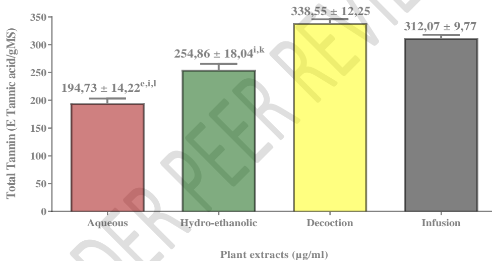
Figure 13 : Concentration of Tannin in plant extracts
