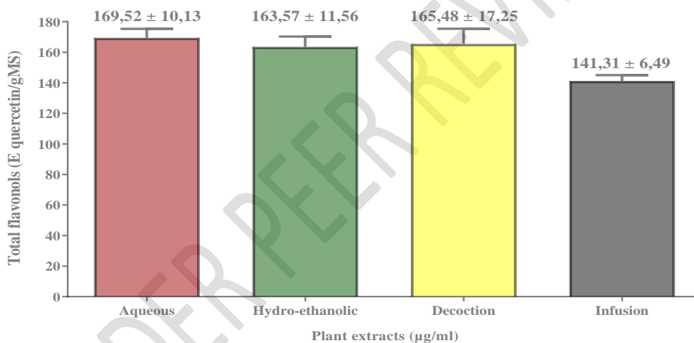
Figure 11 : Concentration of flavonols in plant extracts
