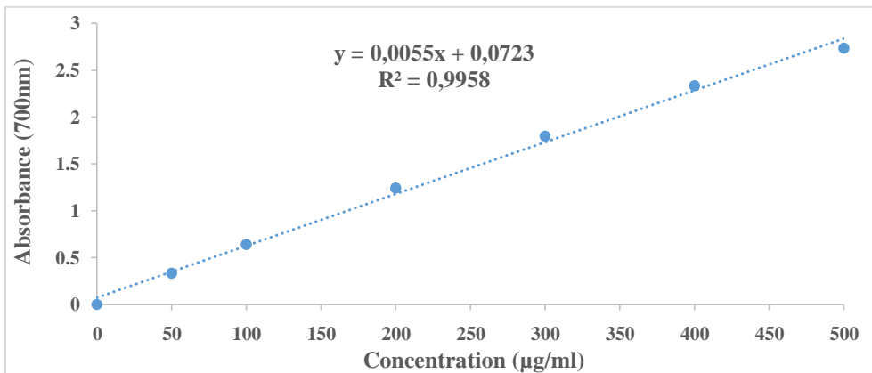
Figure 12 :Calibration curve of Tannic acid
