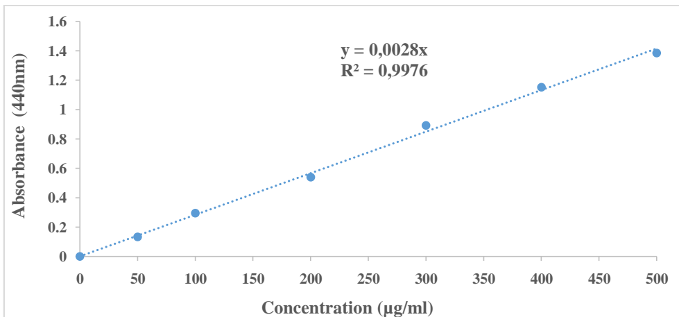
Figure 10 : Calibration curve of quercetin
