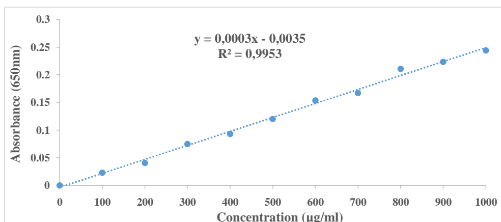
Figure 14: Calibration curve of quinine
