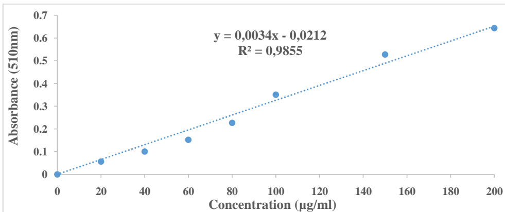
Figure 8 : Calibration curve of quercetin
