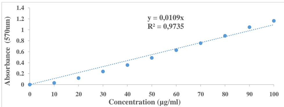
Figure 2 : Calibration curve of glucose.
