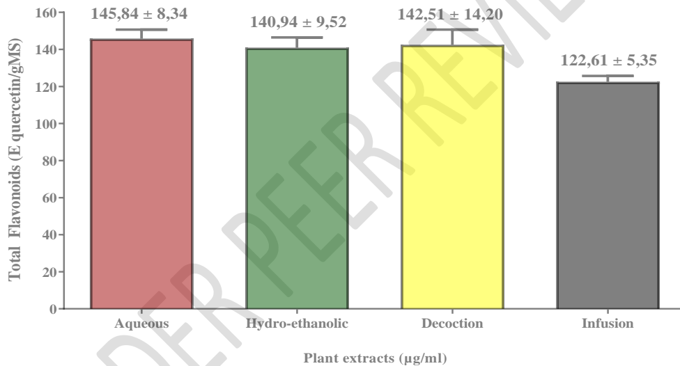
Figure 9: Concentration of Flavonoids in plant extracts
