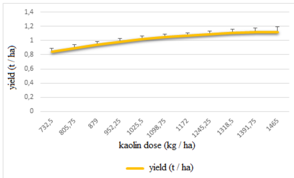
Figure 1: Regression curve of rice response surface to increasing doses of kaolin (Error bar = standard deviation)
