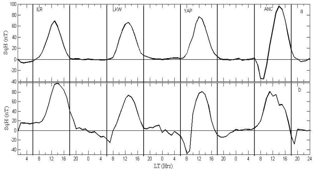
Figure 1. Longitudinal variation of solar quiet Sq H at some selected equatorial stations across the globe on (a) 30 January, 2008, (b) 31 January, 2008
