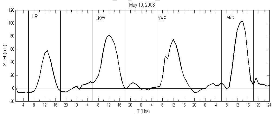
Figure 2. Longitudinal variation of the equatorial electrojet current the quiet day of May 10, 2008
