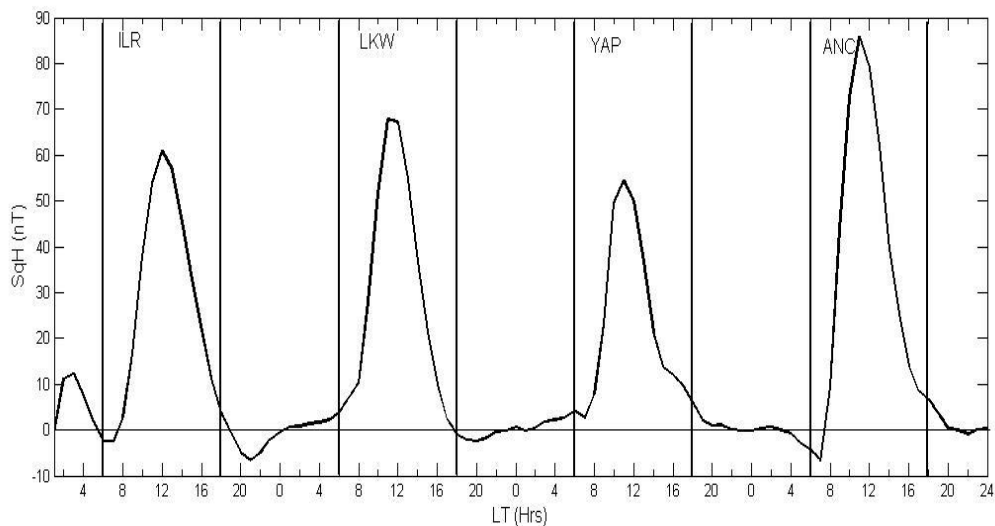
Figure 4. Diurnal variation of H-field on November 4, 2008
