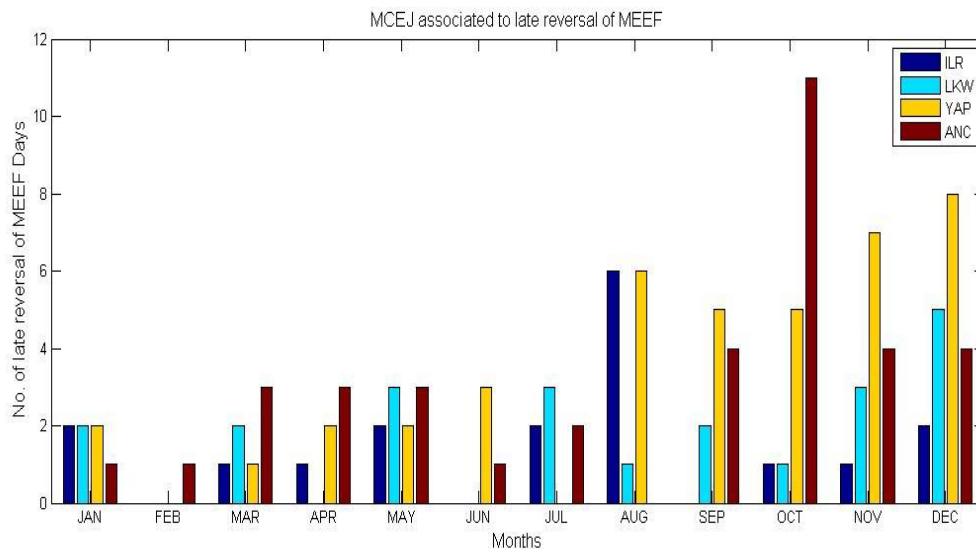
Figure 7. Occurrence of late reversal of morning eastward electric field (MEEF)
