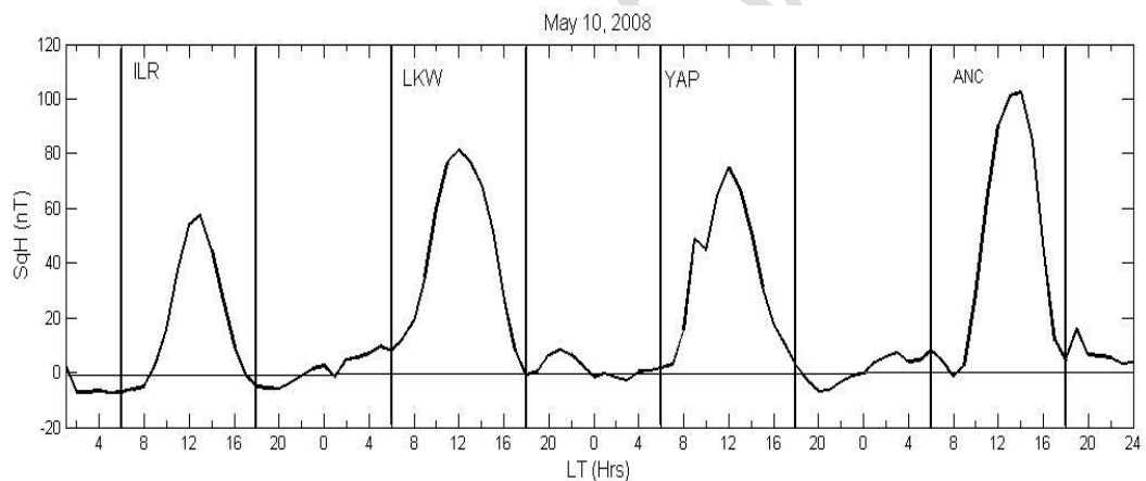
Figure 2. Diurnal variation of the EEJ on May 10, 2008
