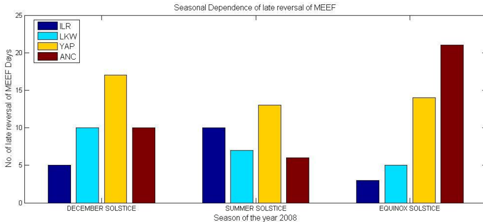
Figure 8b. Seasonal variation of late reversal of MEEF in year 2008.
