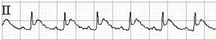
Figure 1c. Restraint stress alone group: P is taller indicating delay in atrial depolarization, T height increased indicating myocardial infarction. Increase in the mean heart rate.
