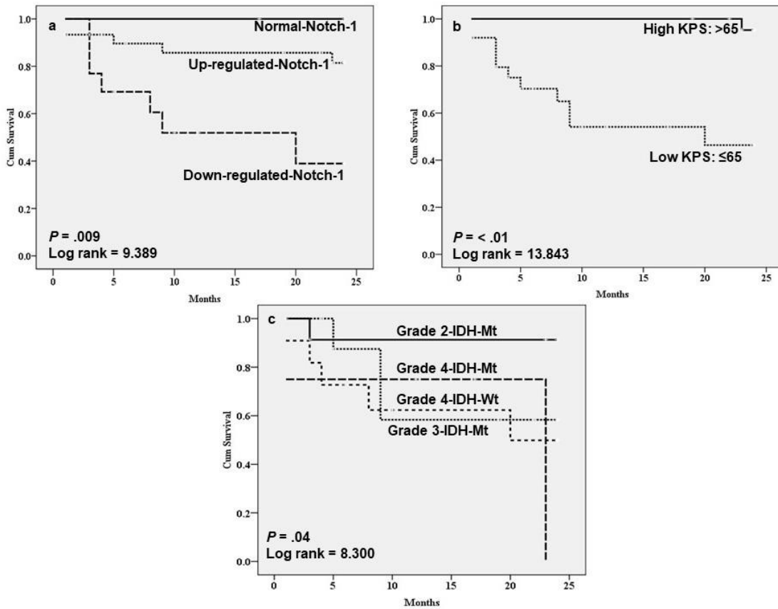
Figure 5. Kaplan-Meier Survival curves for progression-free survival. a. Patients with different Notch1 gene expression b. Patients with KPS score c. Patients with different grade of tumors.
