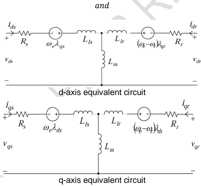
Picture . 2. d-q equivalent circuit of the induction motor[26].
