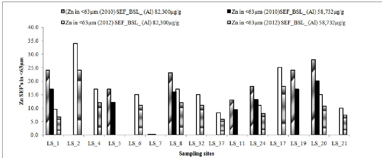
Fig. 5. The calculated SEF for Zn in <63µm grain size fraction of surficial sediments (2012 & 2010 data) using Al baseline values (BSL_Al=82,300µg/g &BSL_Al=58,732µg/g).
