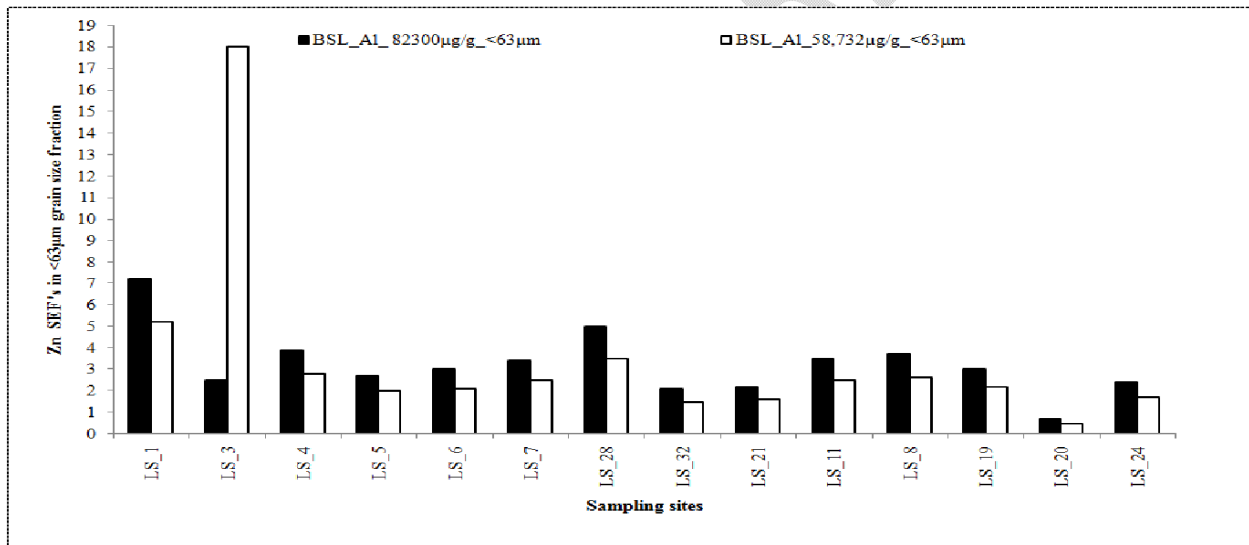
Fig. 7c. The calculated SEF for Zn in <math><63\mu\text{m}</math> grain size fraction of surficial sediments (1994/95 data) using Al (<math>82,300\mu\text{g/g}</math> and <math>58,732\mu\text{g/g}</math>) as a baseline value
