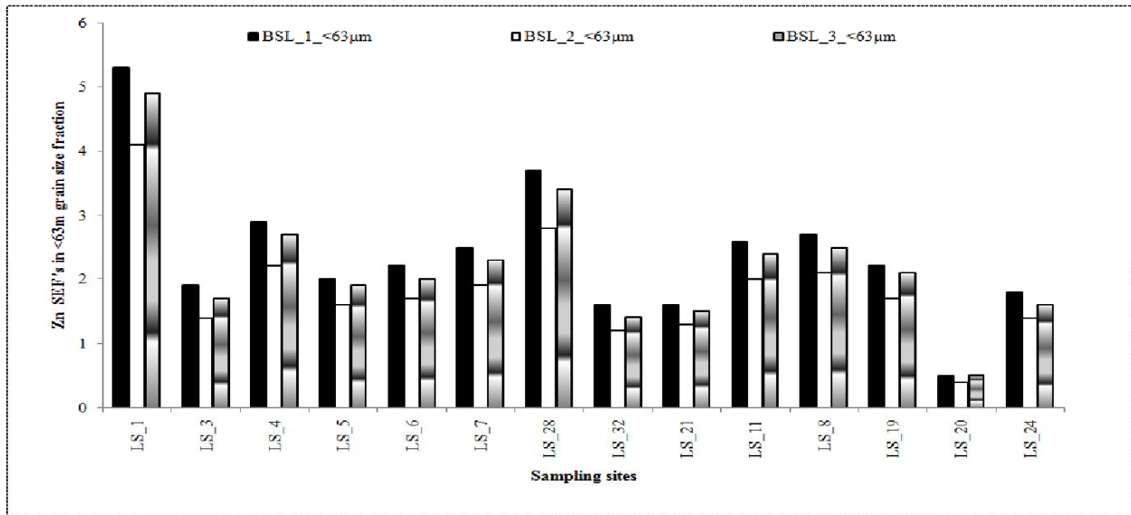
Fig. 7b. The calculated SEF for Zn in <math><63\mu\text{m}</math> grain size fraction of surficial sediments (1994/95 data) using Fe as baseline values (BSL_1=<math>60,800\mu\text{g/g}</math>; BSL_2=<math>46,700\mu\text{g/g}</math>; BSL_3=<math>56,000\mu\text{g/g}</math>).
