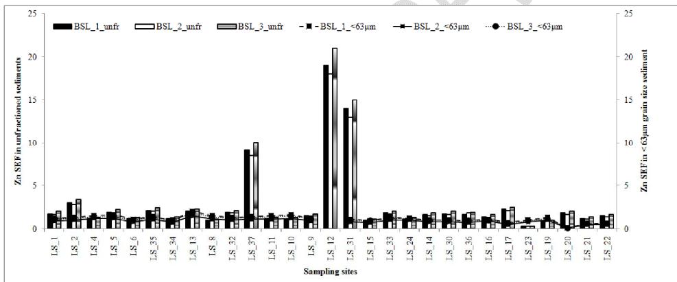
Fig. 7a. The calculated SEF for Zn in un-fractionated (unfr) and <63 \mu\text{m} grain size fraction of surficial sediments (2012 data) using Fe as baseline values (BSL_1= 60,800 & 49,900 \mu\text{g/g} for Fe in <63 \mu\text{m} & un-fractionated sediments respectively; BSL_2=46,700 \mu\text{g/g} ; BSL_3=56,000 \mu\text{g/g} ).
