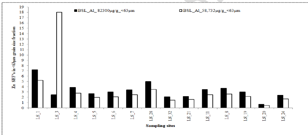
Fig. 7c. The calculated SEF for Zn in <63µm grain size fraction of surficial sediments (1994/95 data) using Al (82300 µg/g and 58,732µg/g) as baseline value
