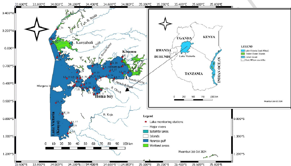
Fig 1. A map of the eastern gulf (Winam or Nyanza gulf) of Lake Victoria (East Africa), showing the sampling stations.
