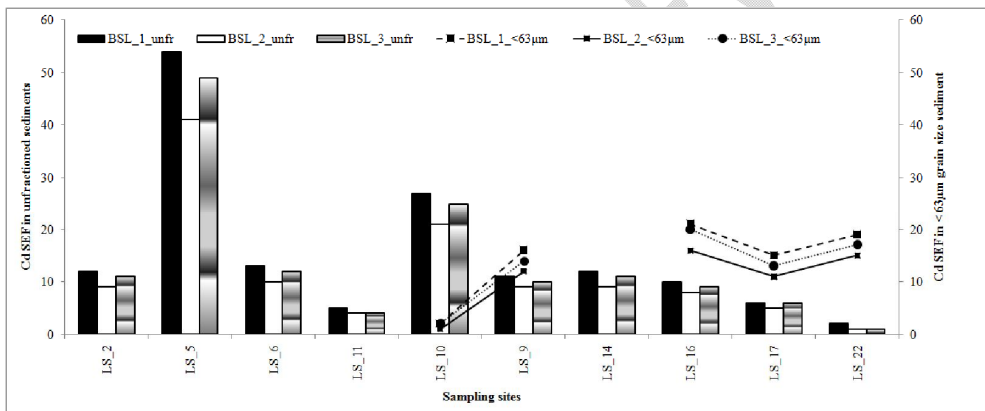
Fig. 6a. The calculated SEF for Cd in un-fractionated (unfr) and <63µm grain size fraction of surficial sediments (2010) using Fe as baseline values (BSL_1=60.800 & 49,900µg/g for Fe in <63µm & un-fractionated sediments respectively; BSL_2=46,700 µg/g; BSL_3=56,000 µg/g).
