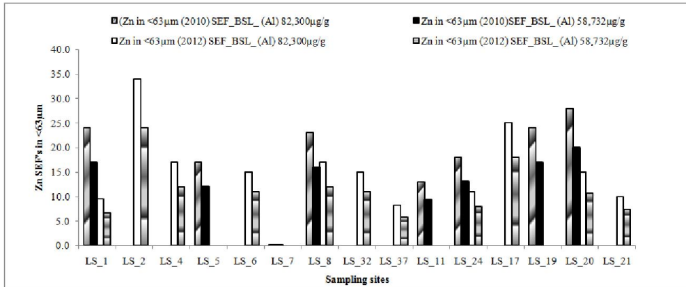
Fig. 5. The calculated SEF for Zn in <63µm grain size fraction of surficial sediments (2012 & 2010 data) using Al baseline values (BSL_AI=82,300µg/g & BSL_AI=58,732µg/g).
