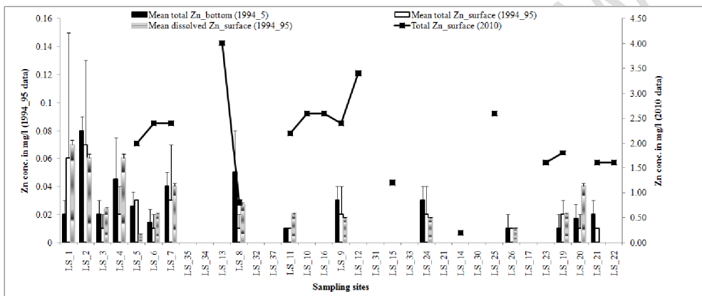
Fig 2. Dissolved and total Zn concentration in surface and bottom waters (2010, 1994/1995 data) of the Nyanza gulf.
