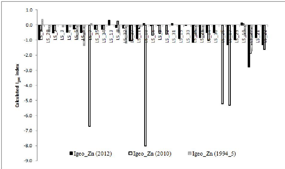
Fig. 4a. Sediment geo-accumulation index (Igeo) values for Zn in < 63µm grain size fraction of the surficial sediments (2012, 2010 & 1994_5 data) in Nyanza gulf.
