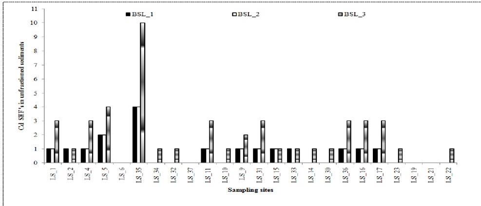
Fig. 6b. The calculated SEF for Cd in un-fractionated surficial sediments (2012) using Fe as baseline values (BSL_1=49,900; BSL_2=46,700 \mu\text{g/g} ; BSL_3=56,000 \mu\text{g/g} ).
