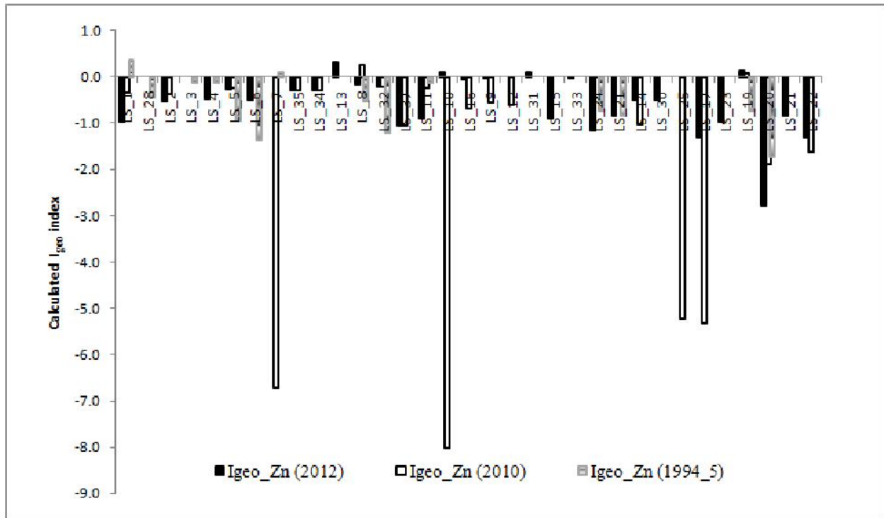
Fig. 4a. Sediment geo-accumulation index (Igeo) values for Zn in < 63 \mu m grain size fraction of the surficial sediments (2012, 2010 & 1994_5 data) in Nyanza gulf.
