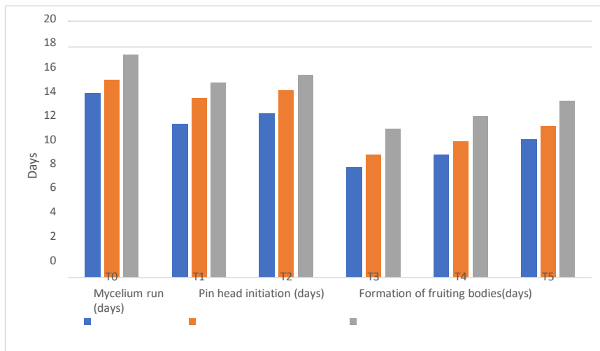
Figure 1. Effect of selected substrates on number of days taken for mycelium run, pin head initiation and fruiting body formation
