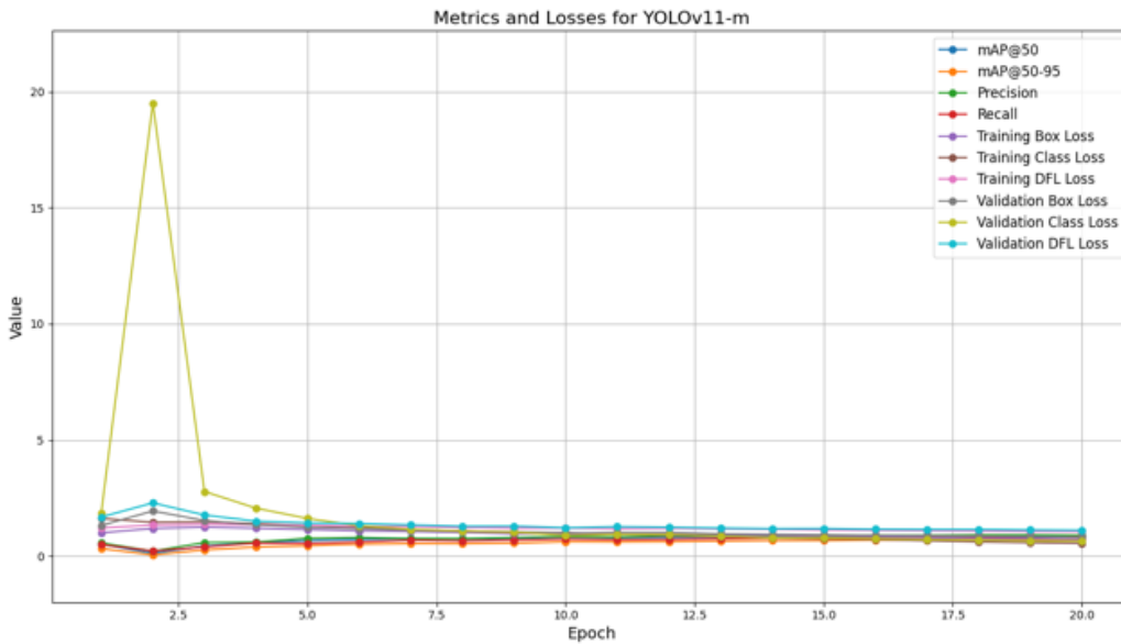
Figure 6: Yolov11-m training
