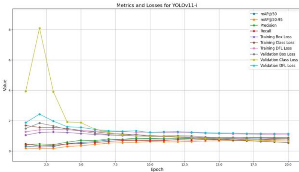
Figure 7: Yolov11-i training
