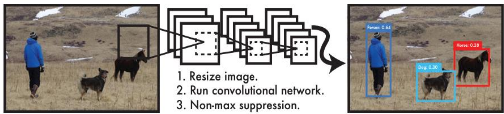
Figure 1: The YOLO Detection System. Processing images with YOLO is simple and straightforward. Our system (1) resizes the input image to 448 × 448, (2) runs a single convolutional network on the image, and (3) thresholds the resulting detections by the model's confidence.[1]
