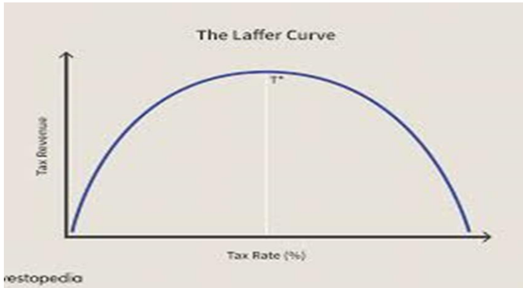
Figure 3 Laffer Curve
