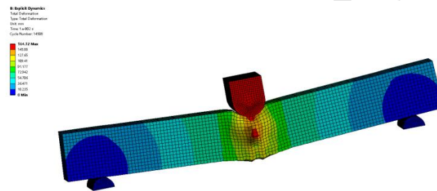
Fig.10 Total deformation cloud image
