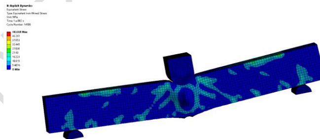
Fig.11 Equivalent stress cloud image
