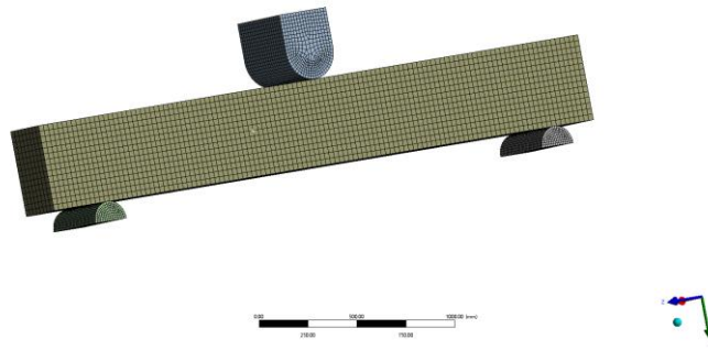
Fig.6 Model grid division diagram
