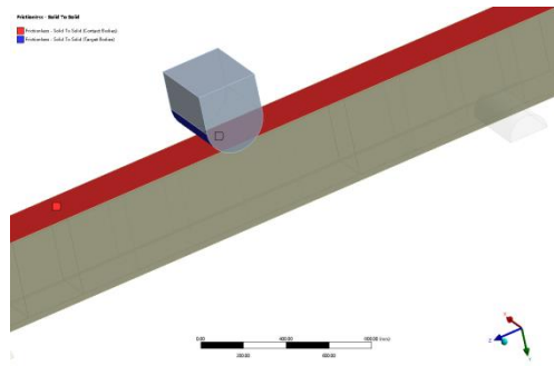
Fig.3 Schematic diagram of contact 1
