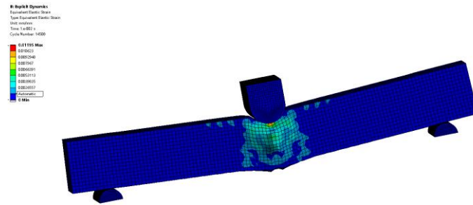
Fig.12 Equivalent elastic strain cloud image
