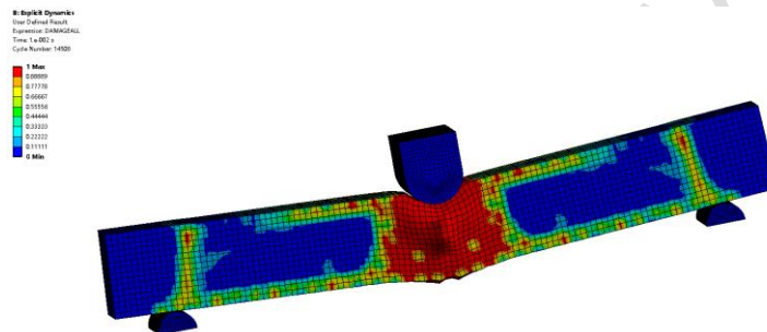
Fig.13 Total destruction cloud image
