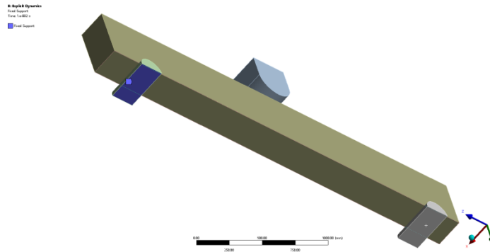
Fig.9 Constraint diagram of fixed end
