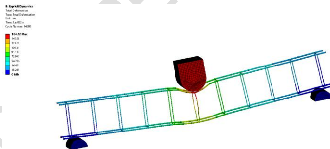
Fig.14 Cloud image of total deformation of steel bars
