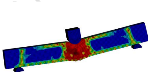
Figure 16 Total destruction cloud image
