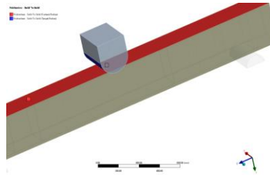
Figure 5 Schematic diagram of contact 1
