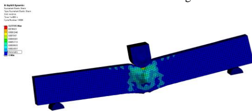
FIG. 15 Equivalent elastic strain cloud image
