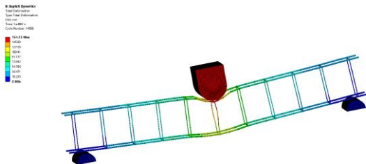
FIG. 17 Cloud image of total deformation of steel bars
