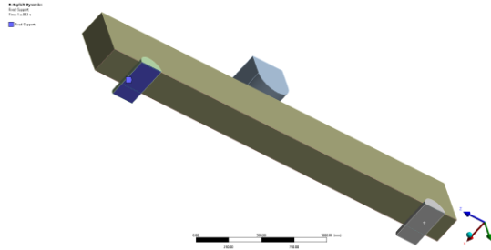
Figure 11 Constraint diagram of fixed end
