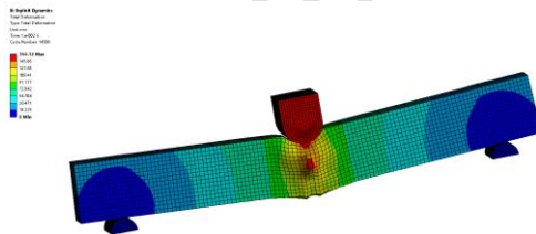
Figure 12 Total deformation cloud image
