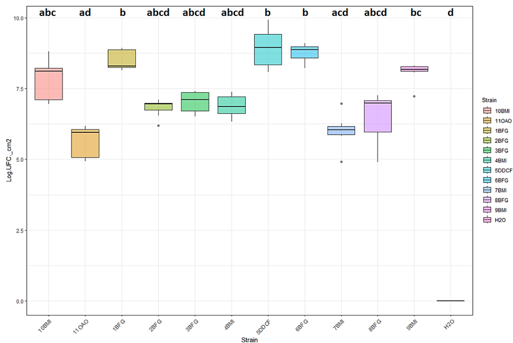
Figure 5: Bacterial population of strains 21 days after inoculation
