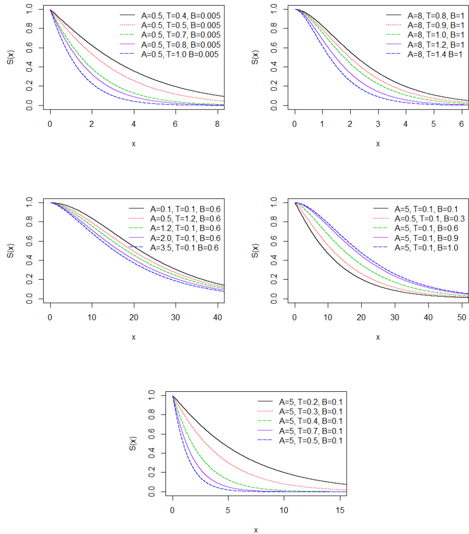
Figure 3: The Survival Function of WQXL distribution
