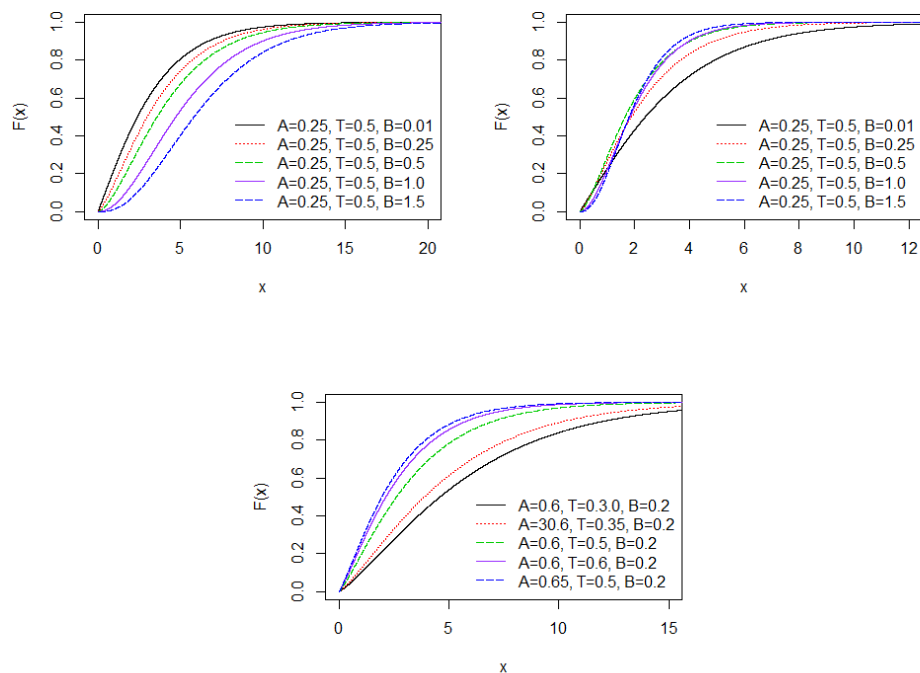
Figure 2: The cumulative distribution function of WQXL distribution
