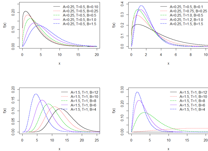
Figure 1: The probability density function of WQXL distribution
