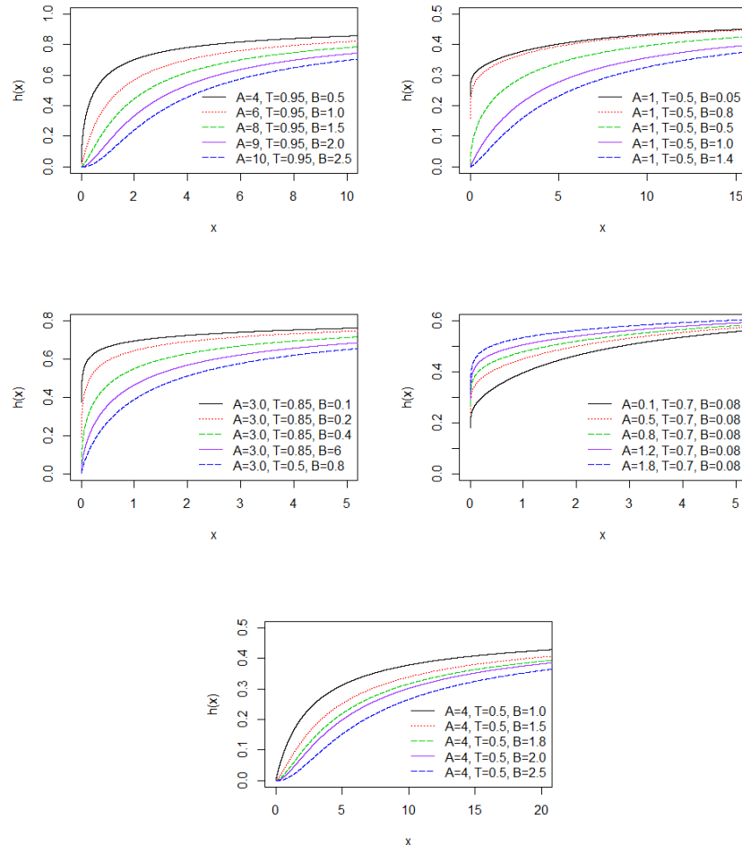
Figure 4: The Hazard Rate Function of WQXL distribution
