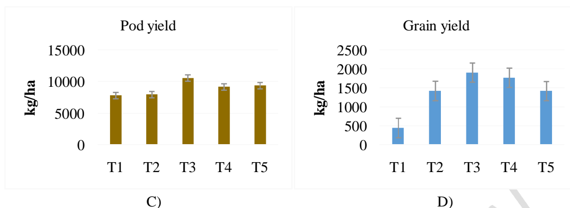
Figure 3. Effect of treatments on yield parameters of cowpea A) effect on test weight B) effect on dry matter production C) effect on pod yield D) effect on grain yield
