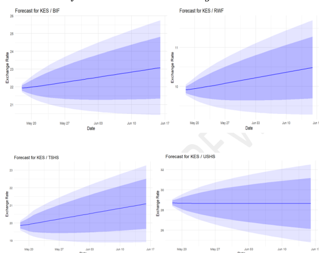
Figure 4: Forecasted Plots for the Hybrid Model
