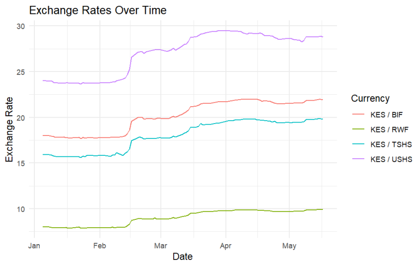
Figure 2: Currency Exchange Rates over Time per Country.
