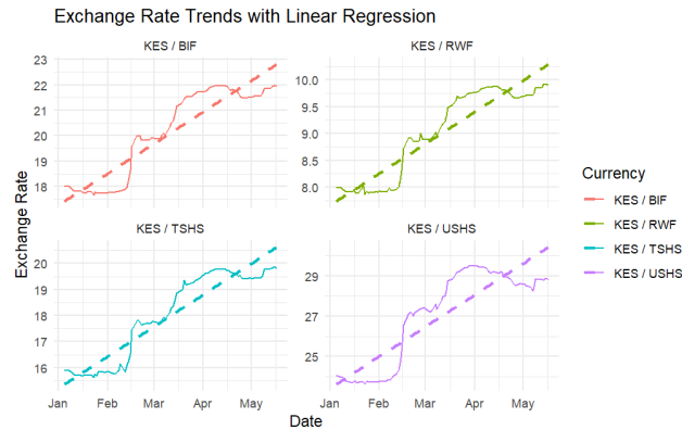
Figure 3: Linear Trend on the Model's Currency Exchange Rates.
