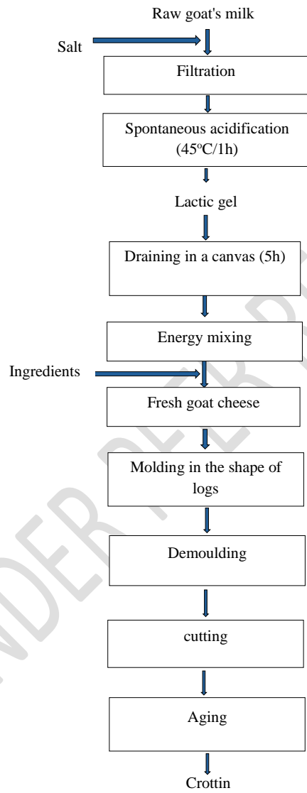
Figure 13: Goat cheese production diagram.
