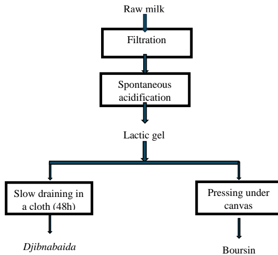
Figure 12: Production diagram for traditional lactic curd cheeses
