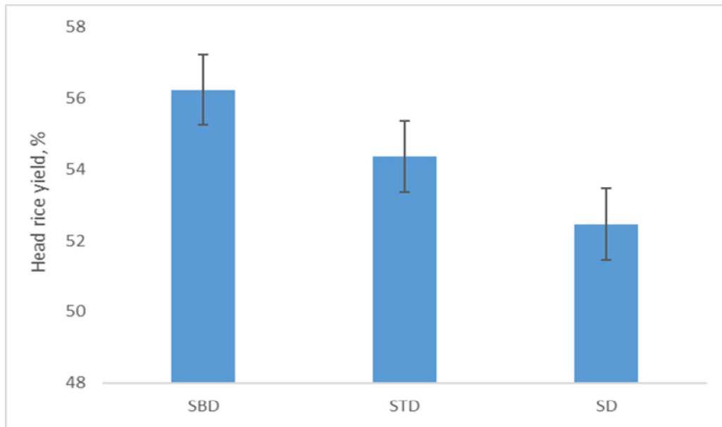
Fig. 5 Variation of head rice yield with different drying methods
