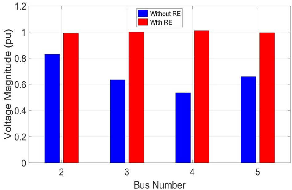
Fig. 7. Bar chart showing the voltage profile without and with RE
