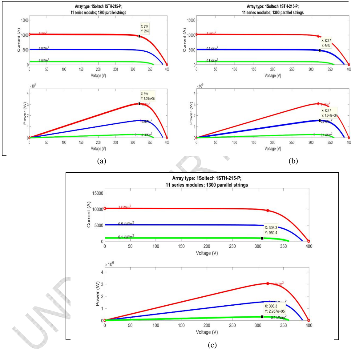
Fig. 5. (a) PV array specification with 1\text{ k W/m}^2 irradiance. (b) PV array specified with 0.5\text{ k W/m}^2 irradiance. (c) PV array specified with 0.1\text{ k W/m}^2 irradiance
