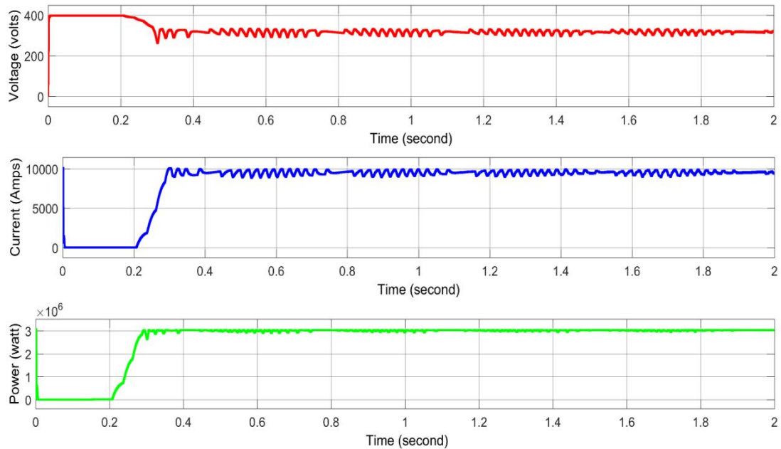
Fig. 6. PV array output current, voltage and power
