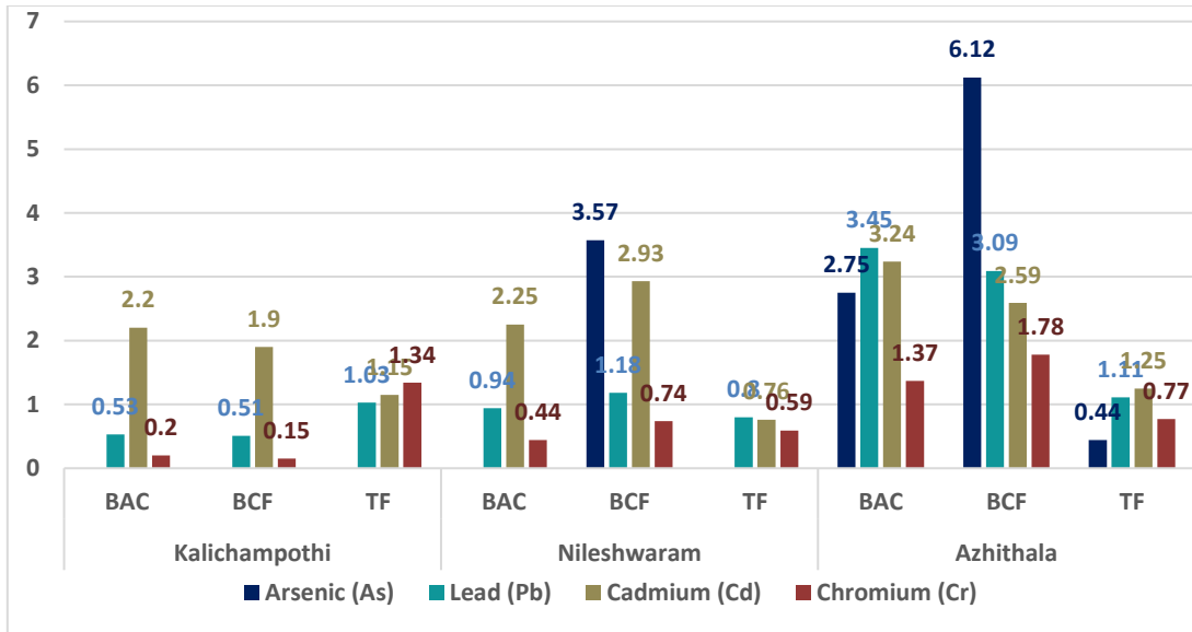
Fig 1: BAC, BCF and TF of Singapore daisy from three location
