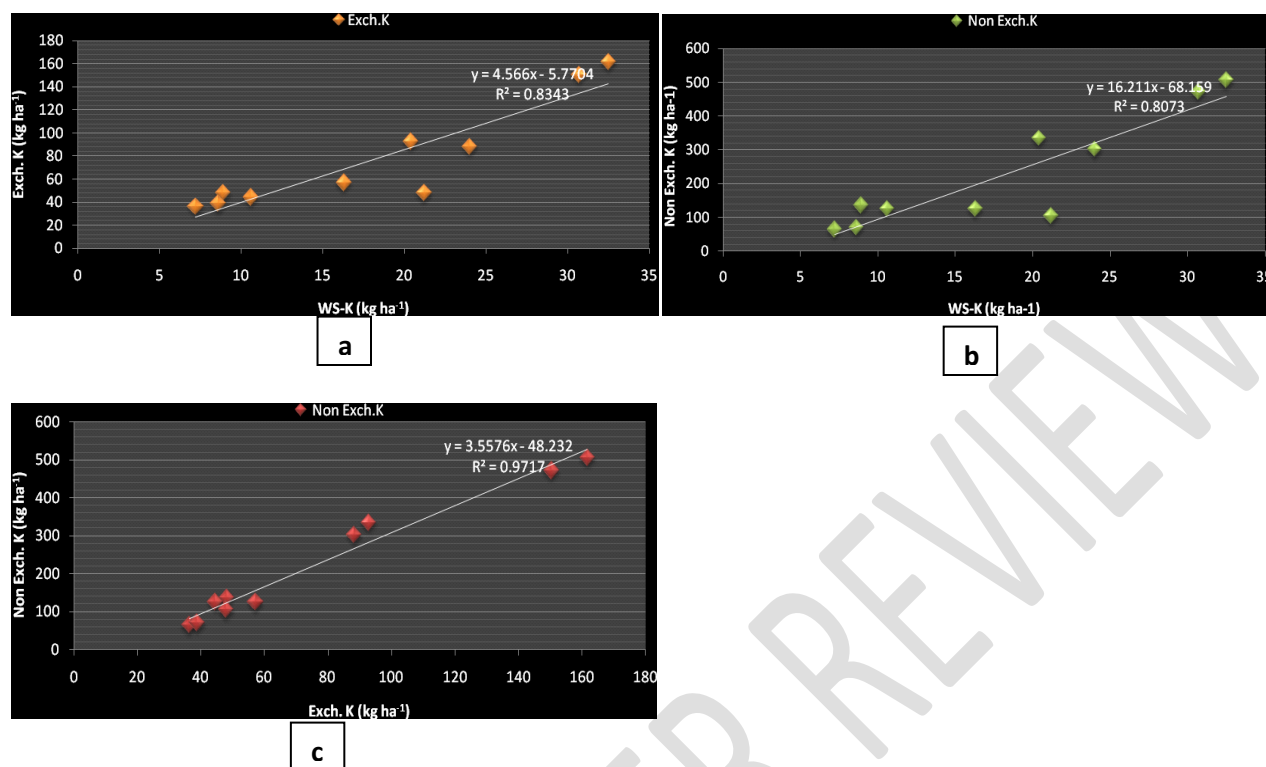
Fig 1: Relationship between (a) WS K vs. exch. K (b) WS K vs. non-exch. K (c) exch. K vs. non-exch. K
