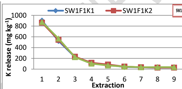
Fig. 3. Potassium release in K 40 treatment
