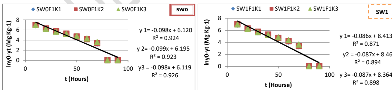
Fig. 7. First order equation kinetics of non-exchangeable K released in K_0 and K_{40} .
