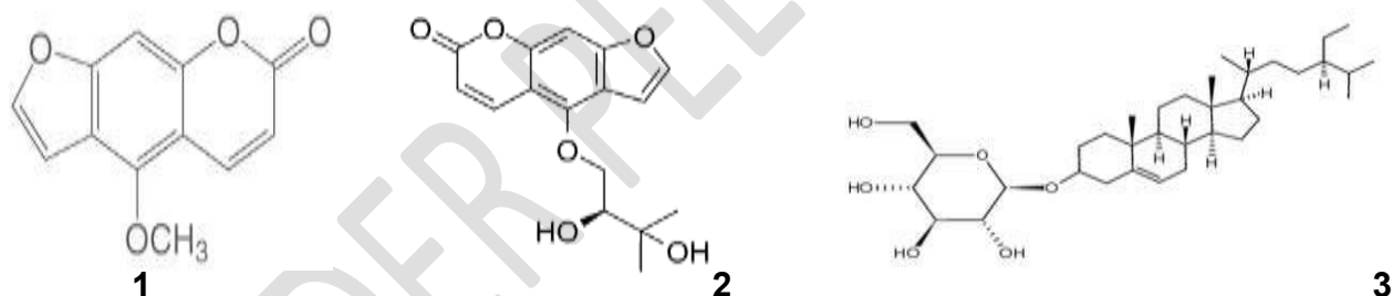
Fig 5. Structure of Bergapten (1), oxypeucedanine hydrate (2) and \beta sitosterol-3-O- \beta -D-glucopyranoside (3).
