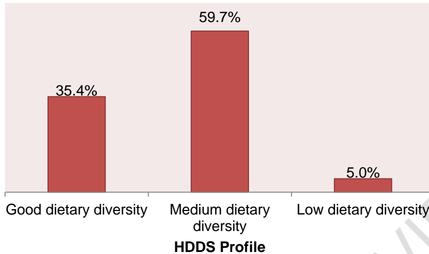
Figure 2: HDDS classification
