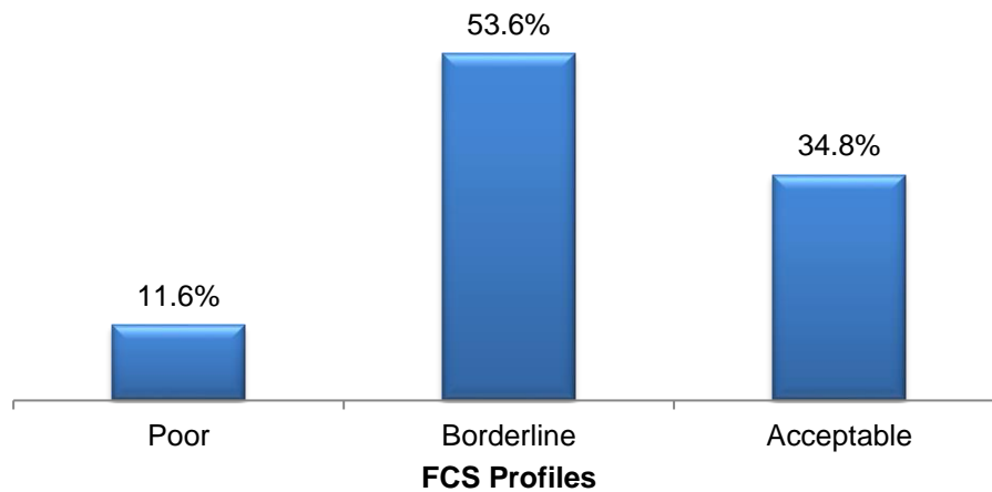
Figure 1: FCS classification
