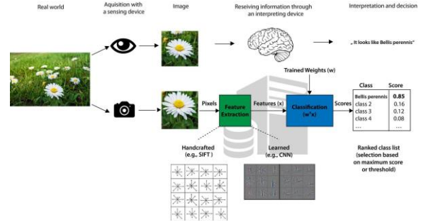
Fig 3: AI Species Identification Workflow
