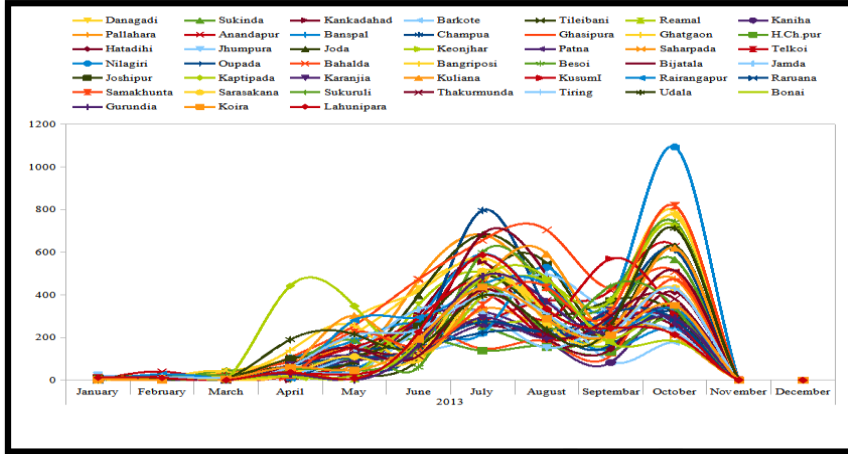
Figure 9: Block wise monthly average rainfall of South Singhbhum Region in 2013
