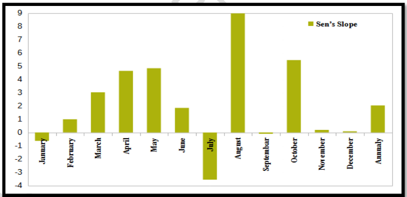
Figure 6: Sen's Slope estimator for the monthly and annual rainfall in the south Singhbhum region
