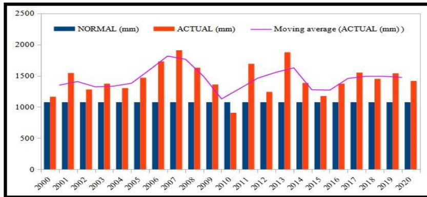
Figure 3.: Comparison between the Normal and Actual Rainfall in Subarnarekha River Basin
