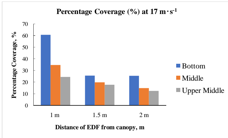
Figure 5. Percentage coverage of spray droplets at different operating conditions of EDF (a) 15 m·s -1 air flow velocity (b) 17 m·s -1 air flow velocity.
