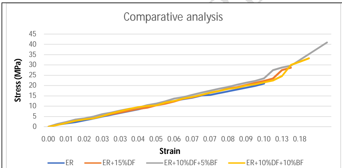
Graph 1&2 :load vs displacement and stress vs strain diagrams for epoxy resin and all developed composite systems
