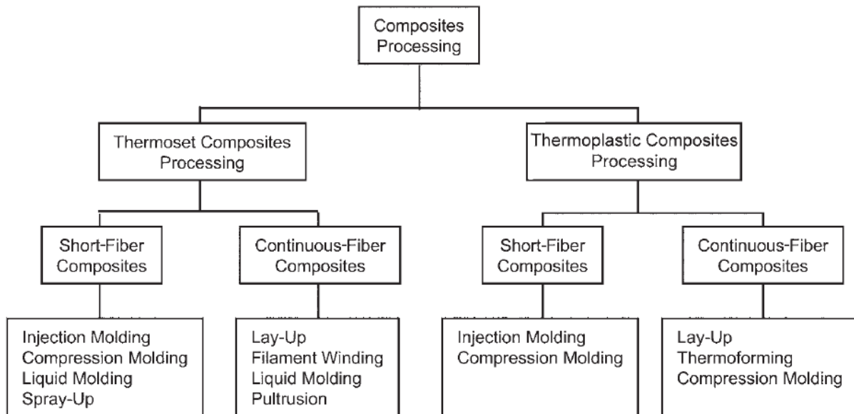
Figure 1: Polymer composites method of formation (Campbell, 2010).
