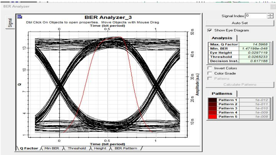
Figure 10: Q Factor and BER values of ONU 3
