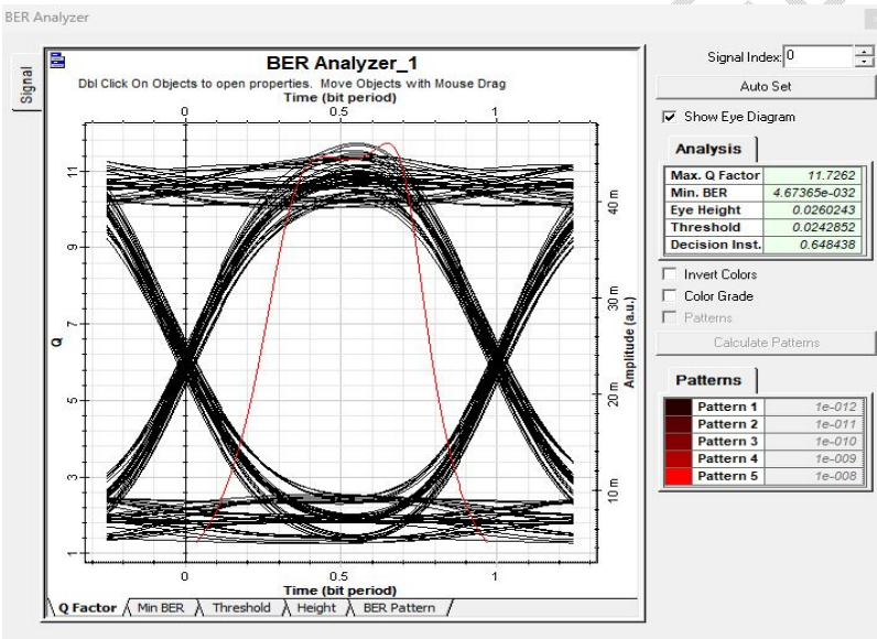
Figure 9: Q Factor and BER values of ONU 2
