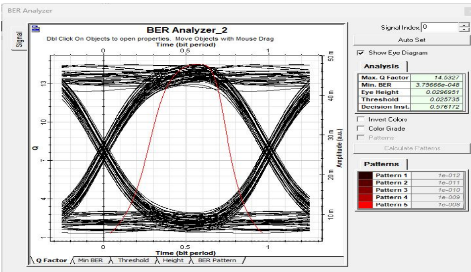
Figure 11: Q Factor and BER values of ONU 4
