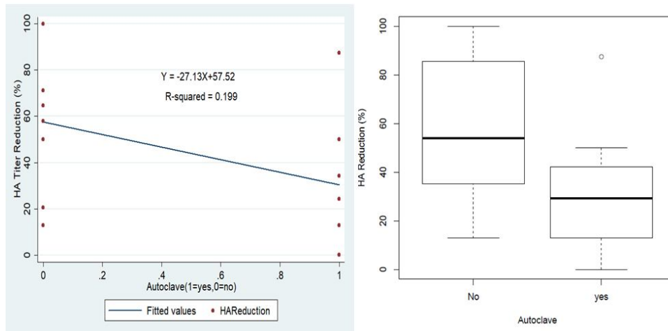
Figure 2: Regression line and box plot reflecting the effect of heat treatment (during autoclaving) on the antiviral activity of studied medicinal plant extracts
