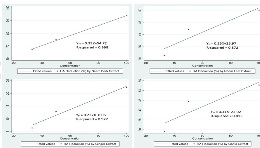
Figure 1: Regression lines reflecting effects of concentration of plant extracts on their anti-viral potential
