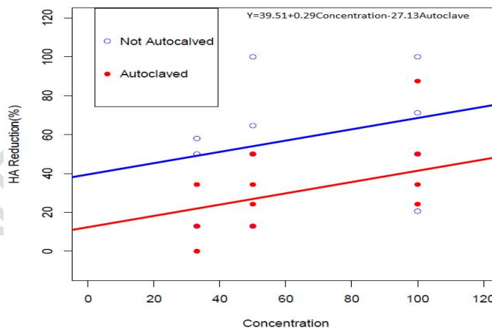
Figure 3: Combined effect of concentration and heat treatment on anti-viral activity of studied medicinal plants
