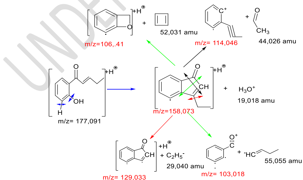
Scheme 1: compound 1 fragmentation mode
