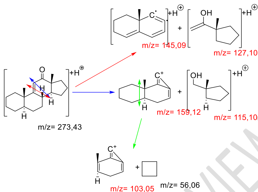
Scheme 10: Compound 10 fragmentation mode
