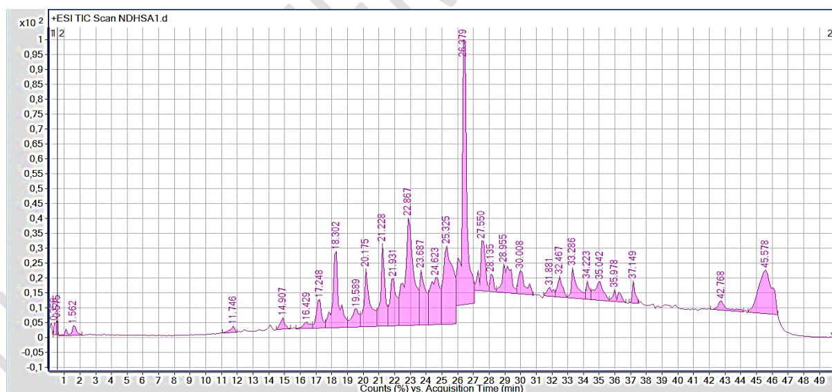
Figure 2: Ethyl acetate fraction major compounds ESI/MS chromatographic profile
