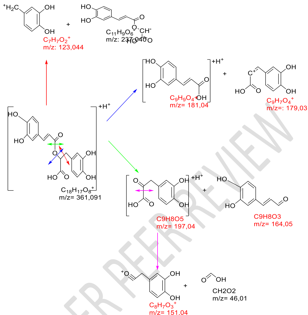
Scheme 15: Compound 15 fragmentation mode
