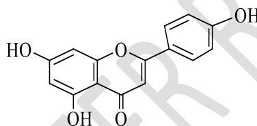
Figure 18 : Structure of compound 8 : Apigenin (5,7-dihydroxy-2-(4-hydroxyphenyl)-4H-chromen-4-one)
