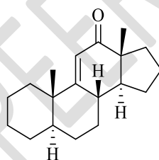
Figure 22 : Structure of compound 10 : 5\alpha -androst-9(11)-en-12-one ((5R,8S,10S,13R,14S)-10,13-dimethyl-1,2,3,4,5,6,7,8,10,13,14,15,16,17-tetradecahydro-12H-cyclopenta[a]phenanthren-12-one)
