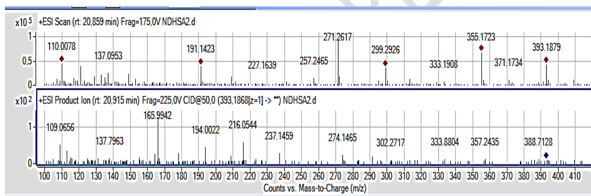
Figure 5: Compound 2 LC-ESI/MS mass spectrum and ESI/MS fragmentation spectrum
