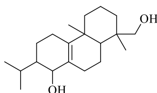
Figure 26 : Structure of compound 12: Suaveolol ( 8-(hydroxymethyl)-2-isopropyl-4b,8-dimethyl-1,2,3,4,4b,5,6,7,8,8a,9,10-dodecahydrophenanthren-1-ol )
