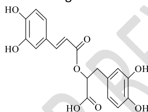
Figure 32: Structure of Compound 15: rosmarinic acid ((E)-3-(3,4-dihydroxyphenyl)-2-((E)-3-(3,4-dihydroxyphenyl)acryloyloxy)propanoic acid)
