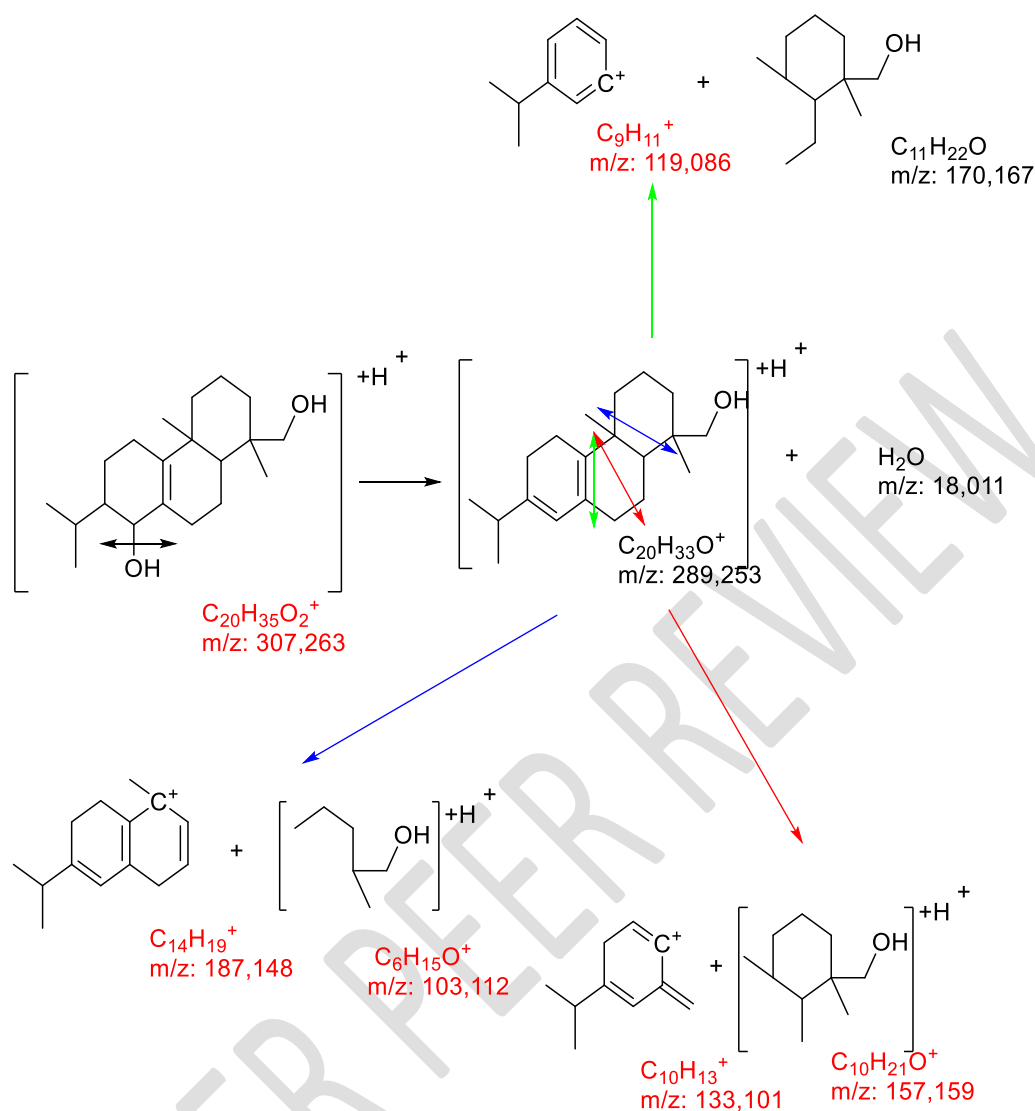
Scheme 12: Compound 12 fragmentation mode
