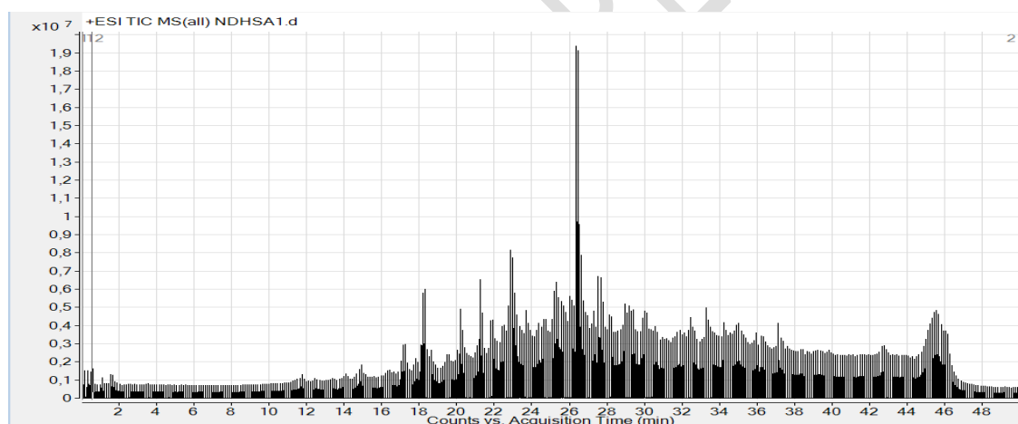
Figure 1: ESI/MS chromatography profile
