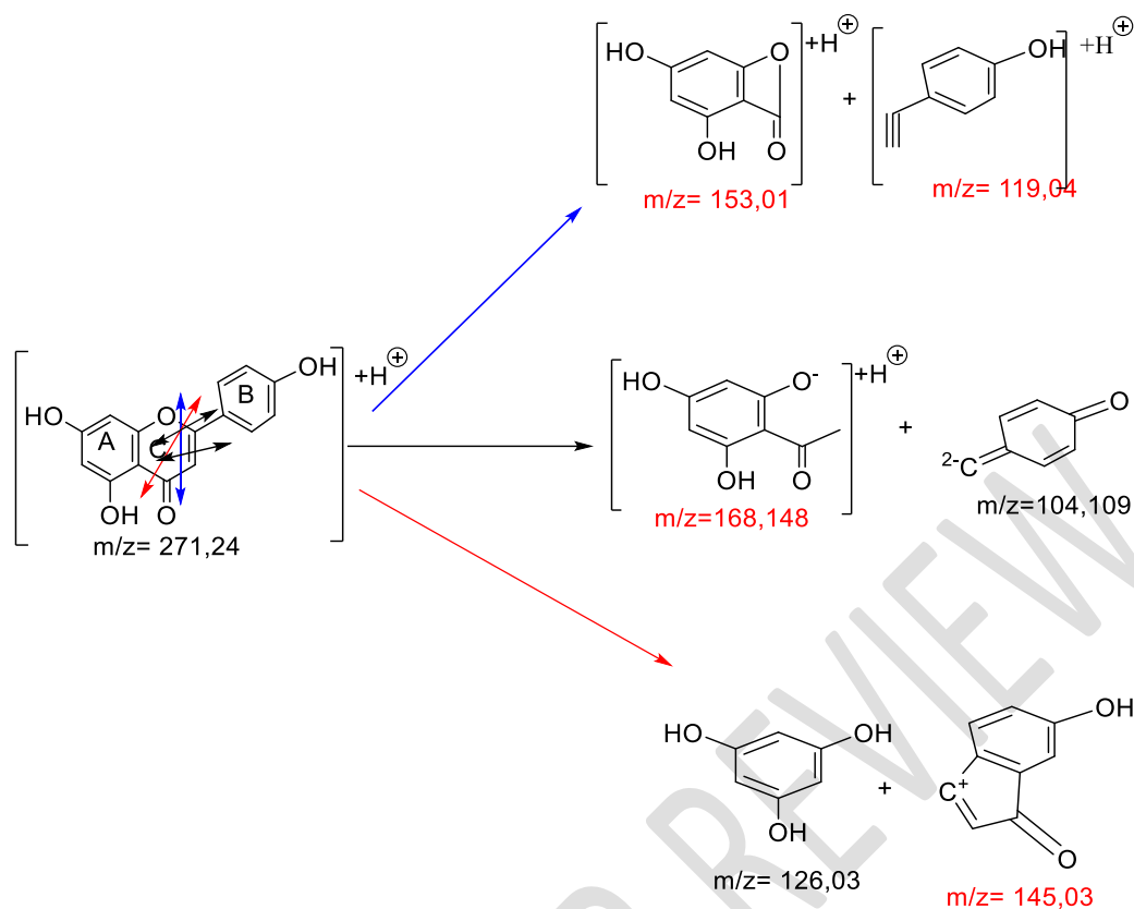
Scheme 8 : Compound 8 fragmentation mode
