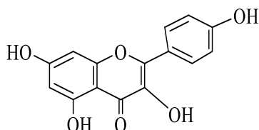
Figure 14 : Structure of compound 6: Kaempferol (3,5,7-trihydroxy-2-(4-hydroxyphenyl)-4H-chromen-4-one)
