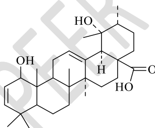
Figure 24: Structure of compound 11 : 1,19 \alpha -dihydroxyl-uros-2(3),12-dien-28-oic acid ((1R,2R,6aS,14bR)-1,12-dihydroxy-1,2,6a,6b,9,9,12a-heptamethyl-1,3,4,5,6,6a,6b,7,8,8a,9,12,12a,12b,13,14b-hexadecahydricene-4a(2H)-carboxylic acid)
