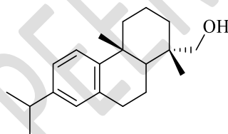
Figure 28: Structure of compound 13: dehydroabietinol ( (((1S,4aR)-7-isopropyl-1,4a-dimethyl-1,2,3,4,4a,9,10,10a-octahydrophenanthren-1-yl)methanol) )
