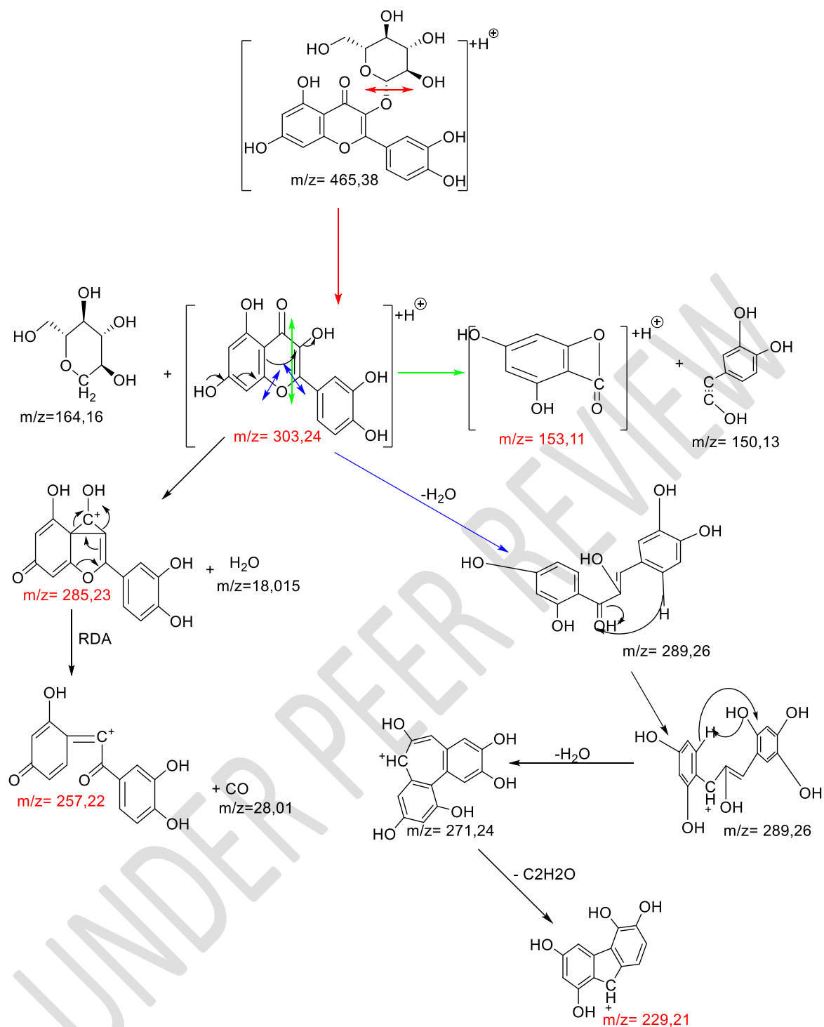
Scheme 4: Compound 4 fragmentation mode
