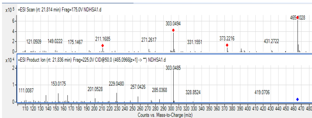
Figure 9 : Compound 4 LC-ESI/MS mass spectrum and ESI/MS spectrum
