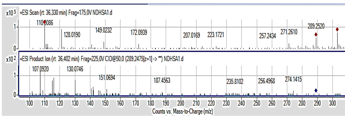
Figure 29 : Compound 14 LC-ESI/MS mass spectrum and ESI/MS fragmentation spectrum
