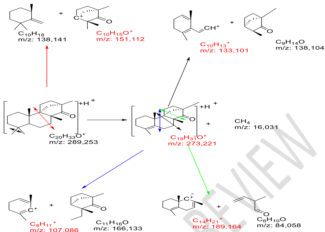
Scheme 14: Compound 14 fragmentation
