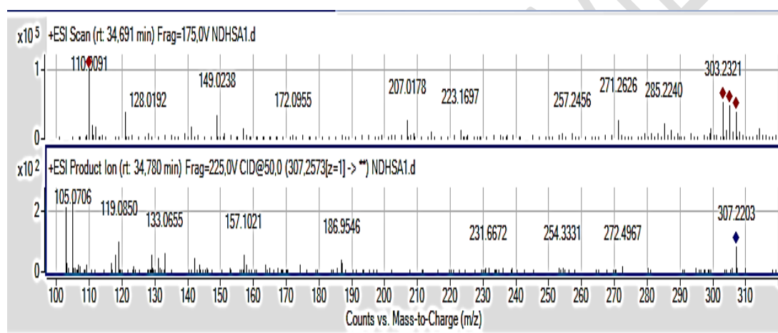
Figure 25 : Compound 12 LC-ESI/MS mass spectrum and ESI/MS fragmentation spectrum
