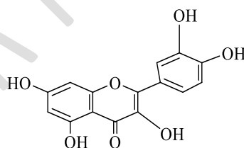
Figure 8 : Structure of compound 3 : quercetin (2-(3,4-dihydroxyphenyl)-3,5,7-trihydroxy-4H-chromen-4-one)
