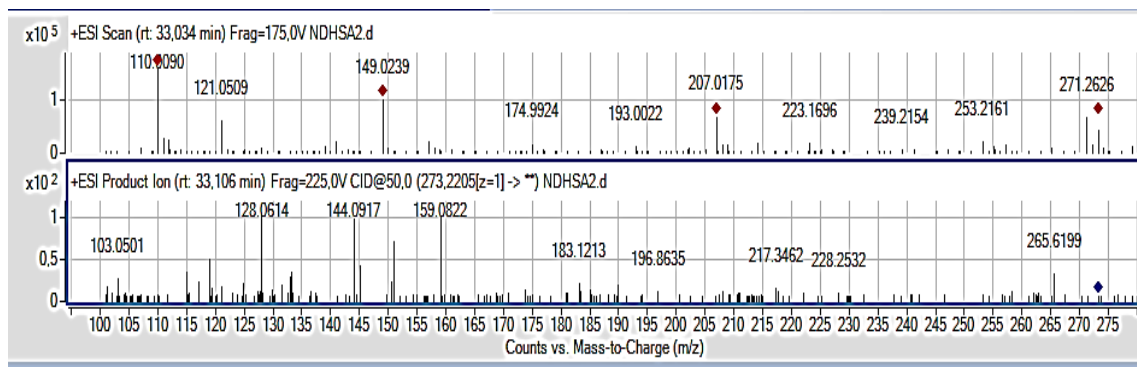
Figure 21 : Compound 10 LC-ESI/MS mass spectrum and ESI/MS fragmentation spectrum
