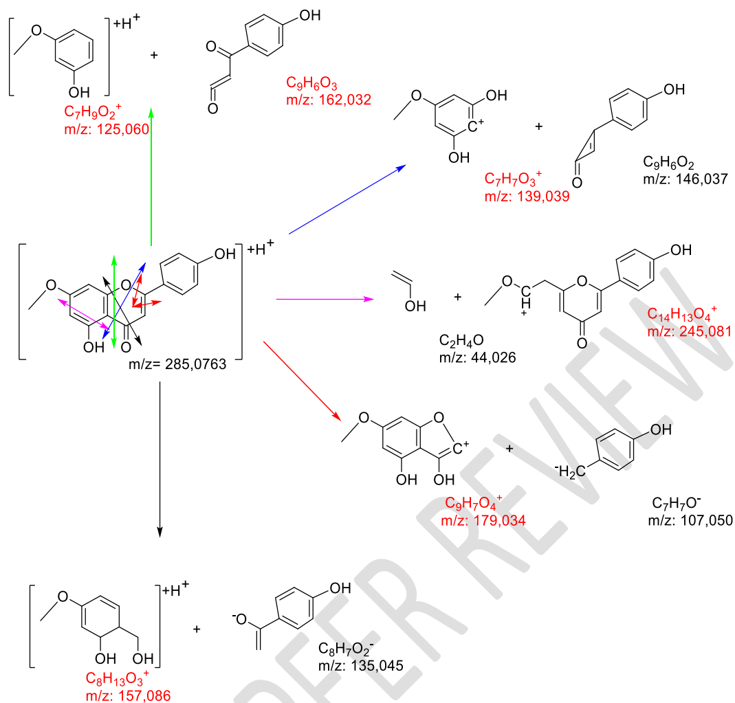
Scheme 9: Compound 9 fragmentation
