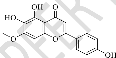
Figure 16: Structure of compound 7: methyl Wogonine (5,6-dihydroxy-2-(4-hydroxyphenyl)-7-methoxy-4H-chromen-4-one)
