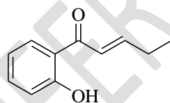
Figure 4: Structure of compound 1 : ((2E)-1-(2-hydroxyphenyl)-pent-2-en-1-one)
