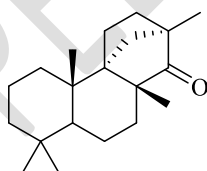
Figure 30 : Structure of Compound 14 ((2R,4aS,4bS,10aR)-2,4b,8,8,10a-pentamethyldecahydro-2H-2,4a-methanophenanthrene-1(4bH)-one)
