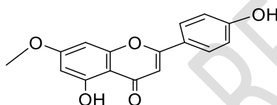
Figure 20 : Structure of compound 9: Genkwanine ( 5-hydroxy-2-(4-hydroxyphenyl)-7-methoxy-4H-chromen-4-one )
