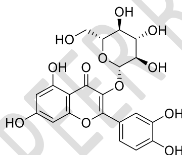
Figure 10: Structure of compound 4 : quercetin 3-O- \beta -D-glucopyranoside ( 2-(3,4-dihydroxyphenyl)-5,7-dihydroxy-3-(((2S,3R,4S,5S,6R)-3,4,5-trihydroxy-6-(hydroxymethyl)tetrahydro-2H-pyran-2-yl)oxy)-4H-chromen-4-one )
