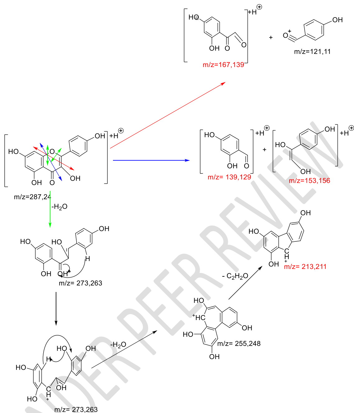
Scheme 6: Compound 6 fragmentation mode
