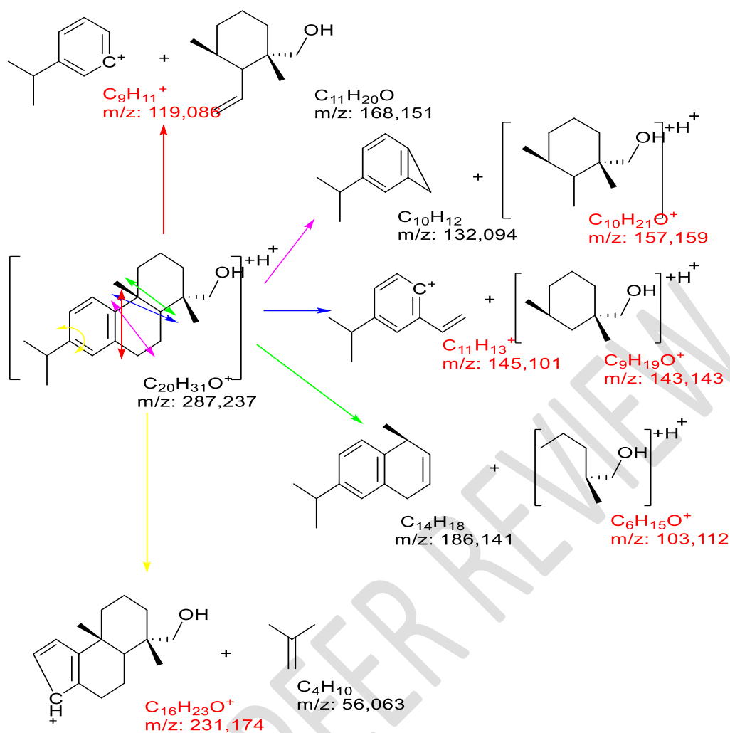
Scheme 13: Compound 13 fragmentation mode
