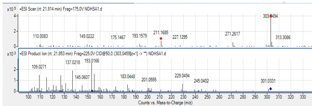
Figure 7 : Compound 3 LC-ESI/MS mass spectrum and ESI/MS spectre de fragmentation spectrm
