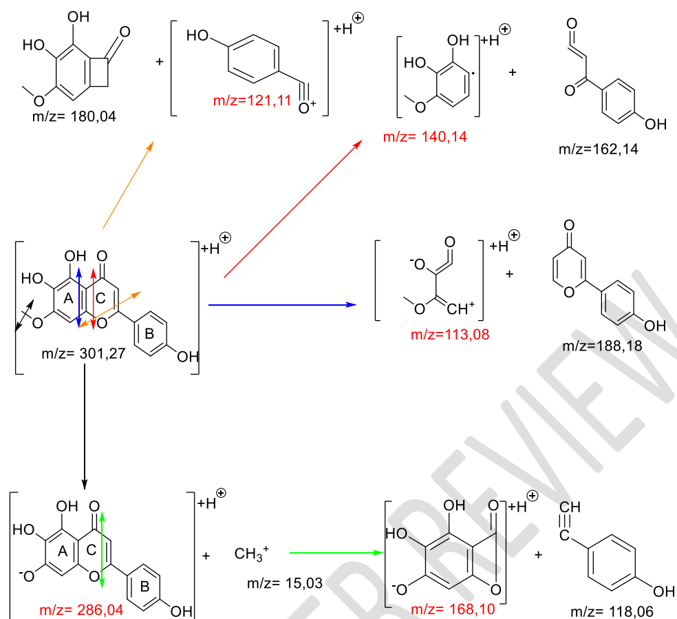
Scheme 7: Compound 7 fragmentation mode
