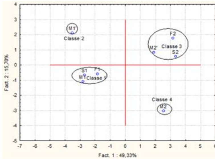
Figure 6: Statistical units space of F1x F2 factorial plan
