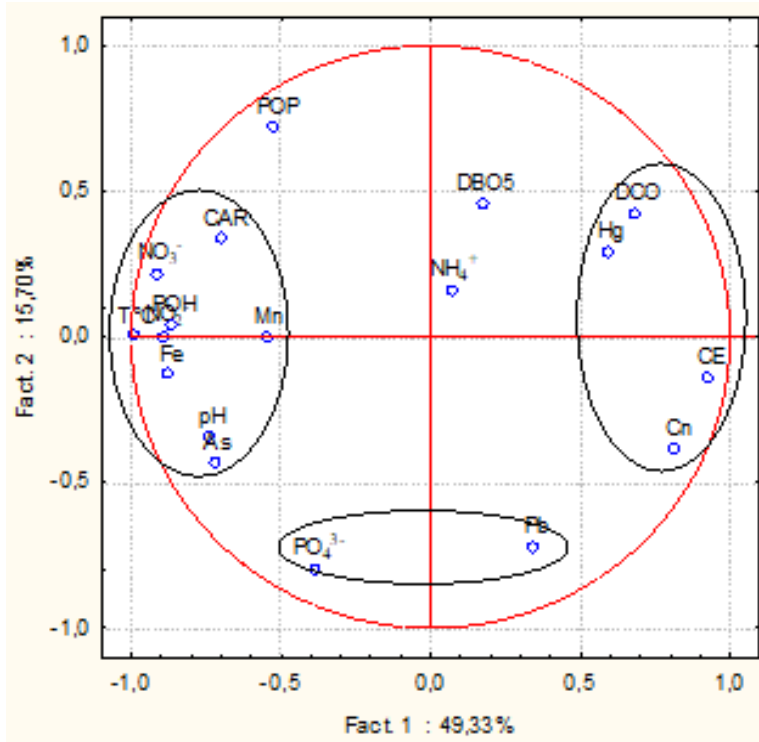
Fig. 5. F1x2 Factorial plan
