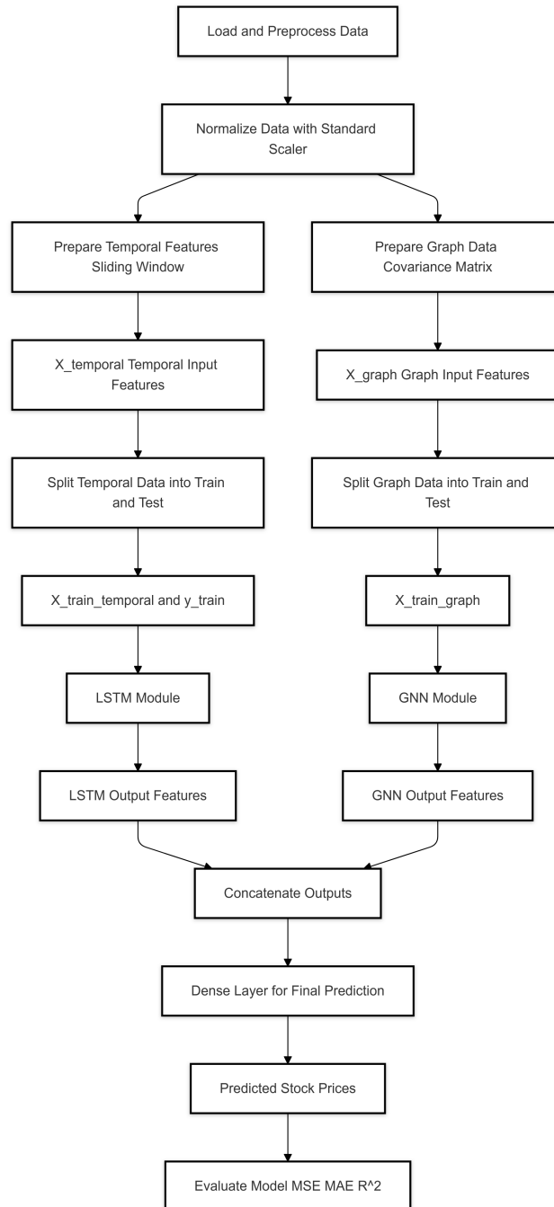
Figure 1: LSTM-GNN Hybrid Model Architecture
