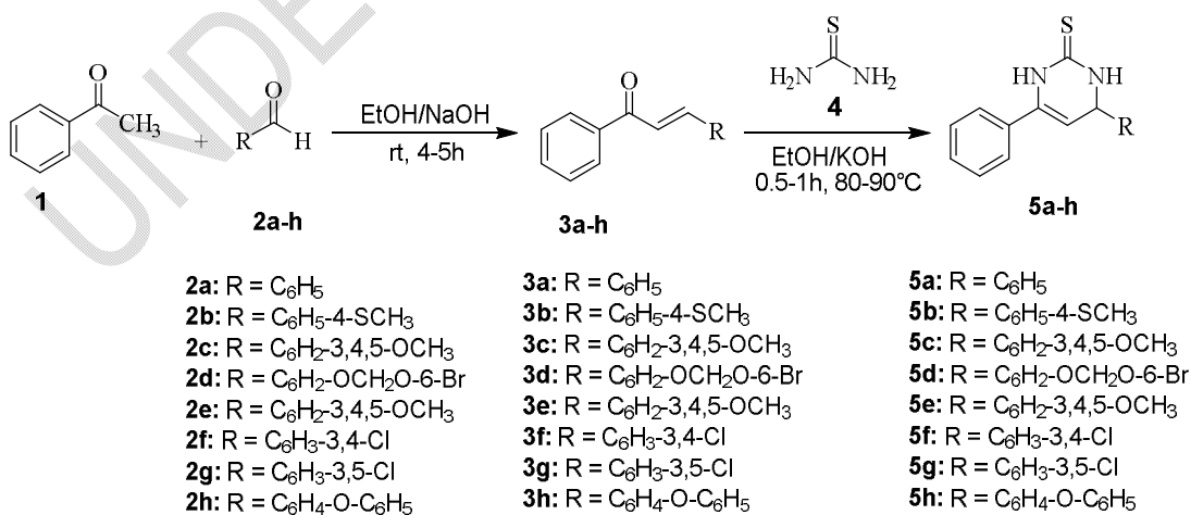
Scheme 1. Synthesis scheme of dihydropyrimidine-2-thiones 5a-h
