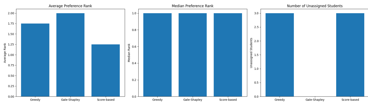
Figure 2: Preference Satisfaction and Unassigned Students by Algorithm
