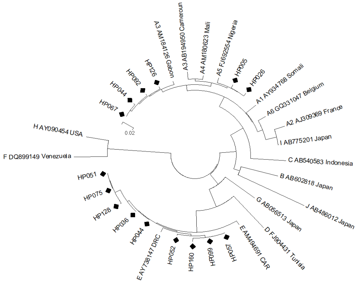
Figure 1. Phylogenetic tree of partial pre-S1 sequences from 15 participants and GenBank references. Bootstrap support values obtained from 1000 replicates are indicated. Accession number and genotype/subgenotype of sequences obtained from GenBank are indicated [CAR, Central African Republic; DRC, Democratic Republic of Congo]. Sequences from this study are in bold font and their name starts with HP.
