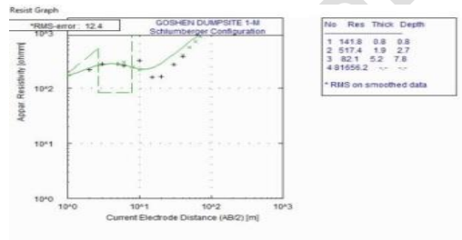
Figure 15: Results of computer modeled curve for VES 12
