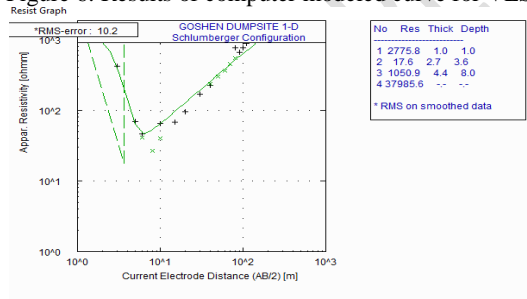
Figure 7: Results of computer modeled curve for VES 4
