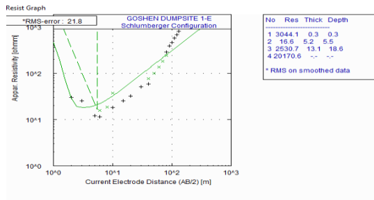
Figure 8: Results of computer modeled curve for VES 5
