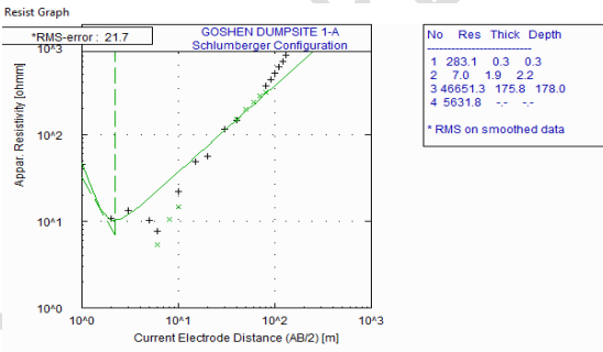
Figure 4: Results of computer modeled curve for VES 1
