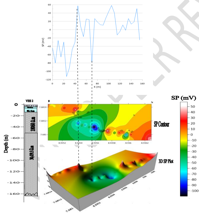
Figure 22: Cross-section correlating the VES transverse, Self-Potential in (mV) signal, SP contours and 3-D SP plot along Profile 2
