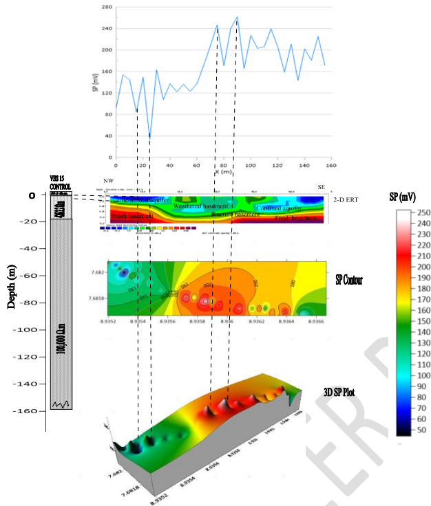
Figure 30: Cross-section correlating the VES transverse, Self-Potential in (mV) signal, SP contours and 3-D SP plot along the Goshen Control Centre
