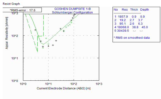
Figure 5: Results of computer modeled curve for VES 2
