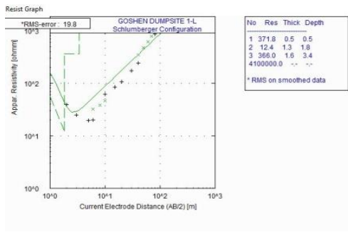
Figure 16: Results of computer modeled curve for VES 13
