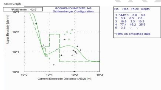
Figure 10: Results of computer modeled curve for VES 7
