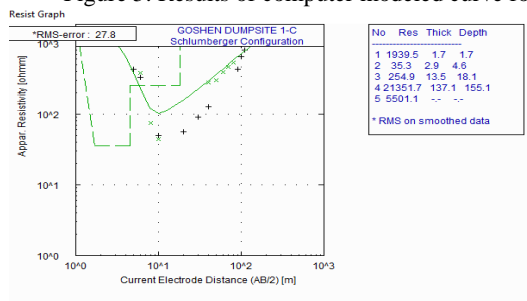
Figure 6: Results of computer modeled curve for VES 3
