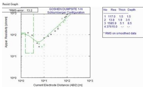
Figure 17: Results of computer modeled curve for VES 14
