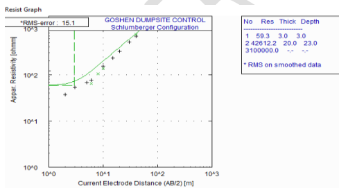
Figure 18: Results of computer modeled curve for VES 15 (Control)
