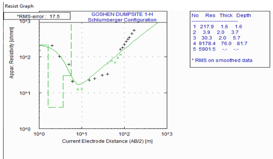
Figure 11: Results of computer modeled curve for VES 8
