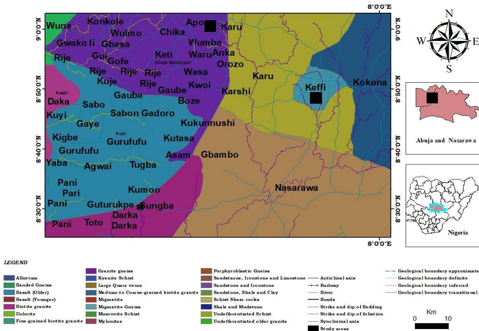
Figure 3: Geological map of the study areas [10]
