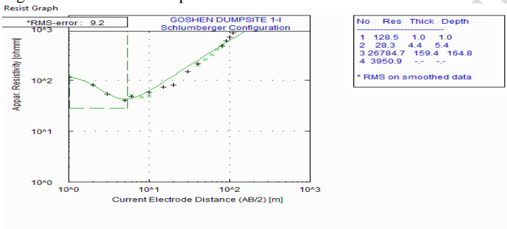
Figure 12: Results of computer modeled curve for VES 9
