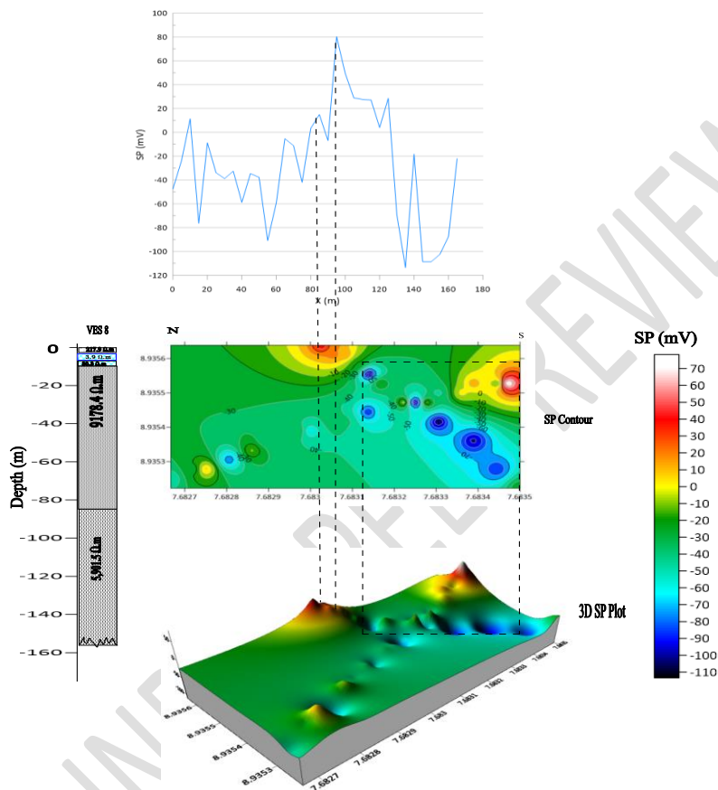
Figure 28: Cross-section correlating the VES Log, Self-Potential in (mV) signal, SP contours and 3-D SP plot along Profile 8
