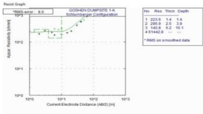
Figure 14: Results of computer modeled curve for VES 11
