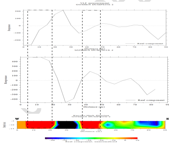
Figure 32: Cross-section of Fraser Filtered, measured VLF and K-H pseudo section along Transverse 2
