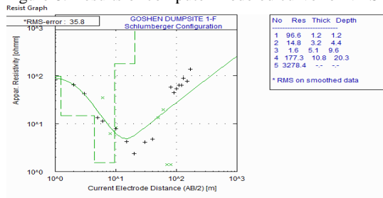
Figure 9: Results of computer modeled curve for VES 6
