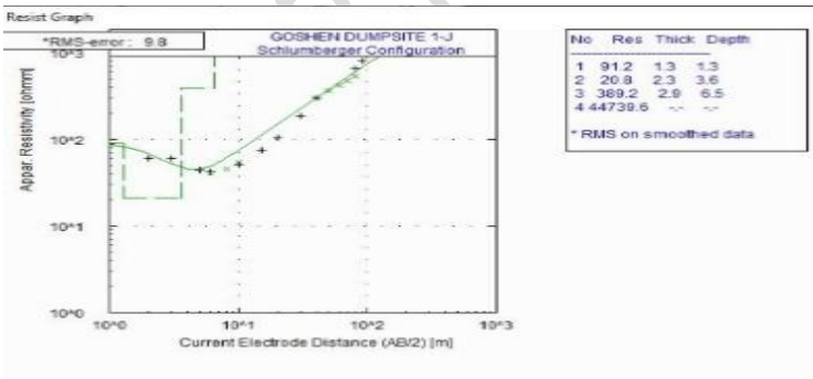
Figure 13: Results of computer modeled curve for VES 10
