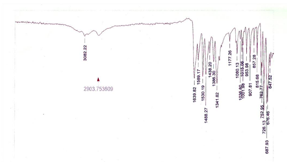
Figure (2): I.R spectrum of N-Phenyl-N-m-nitro benzo hydroxmic acid
