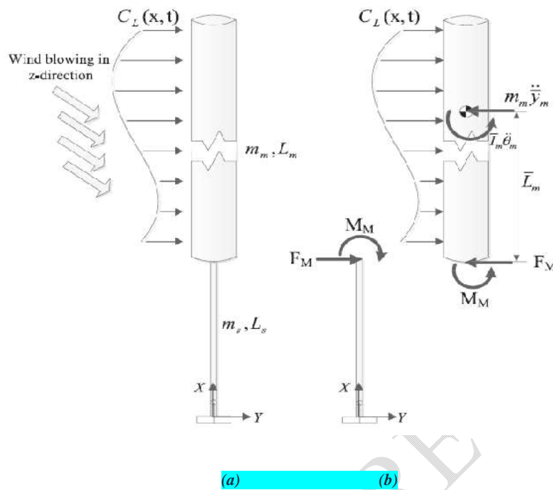
Figure 9:(a) Schematic model of BWT (b) Free body diagram (chizfahm et al. 2008)[24]
