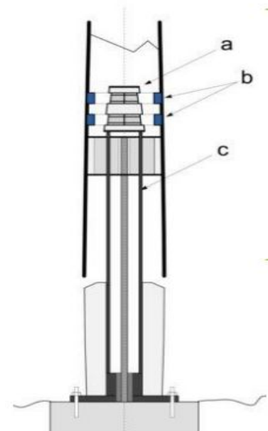
Figure 7: Schematic diagram of BWT Working principle (Vortex Bladeless S.L., 2018)[18]
