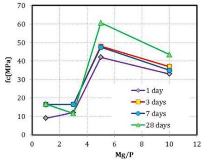
Fig.5 Effect of M/P on compressive strength of MPC [30]
