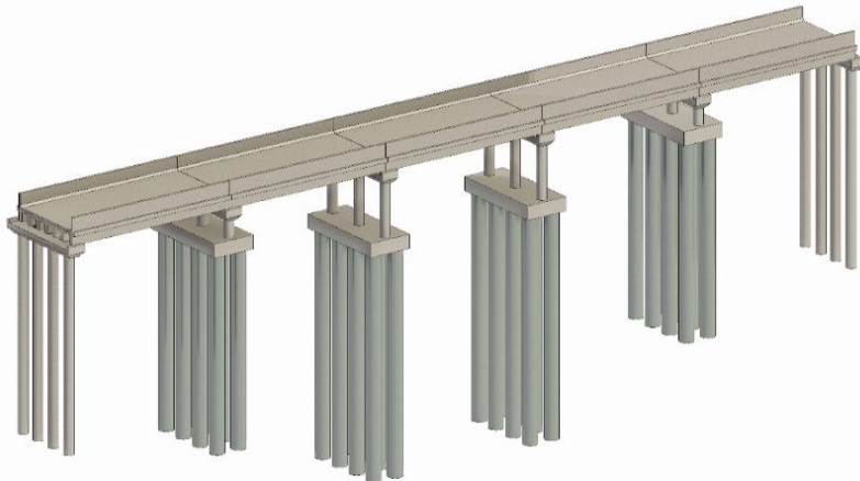
Fig. 8. Revit model of rectangular aqueduct superstructure
