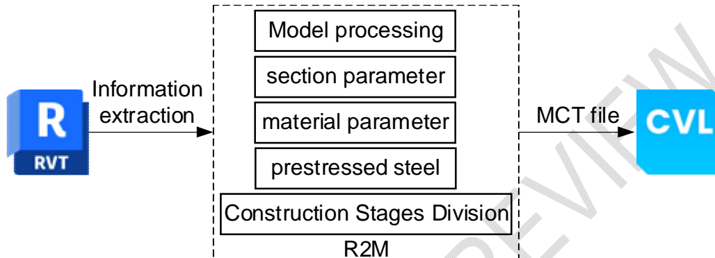
Fig. 1 Revit-Midas model conversion methodology
