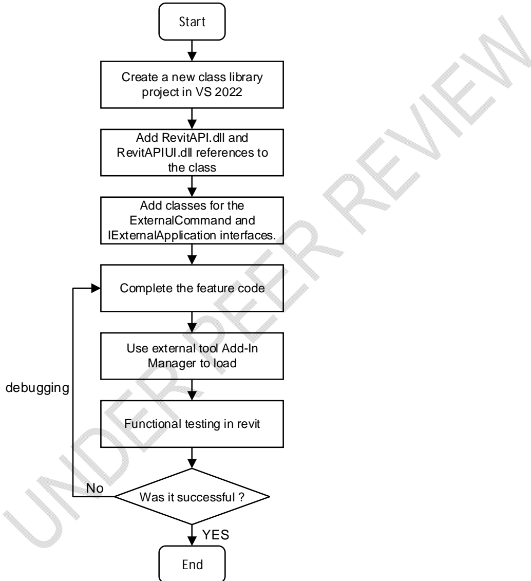
Fig. 2 Secondary development flow chart
