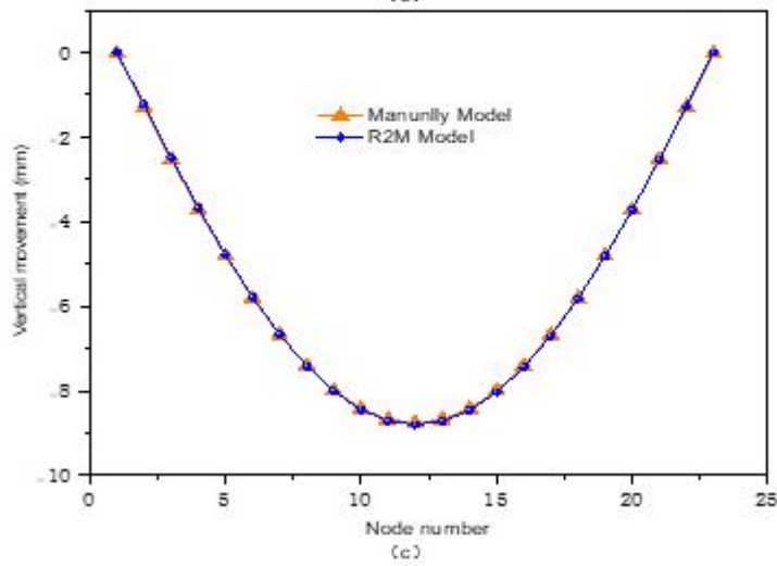
Fig. 9. Vertical displacement calculation results (a) R2M conversion model calculation results (b) Midas manual modelling calculation results (c) Model comparison
