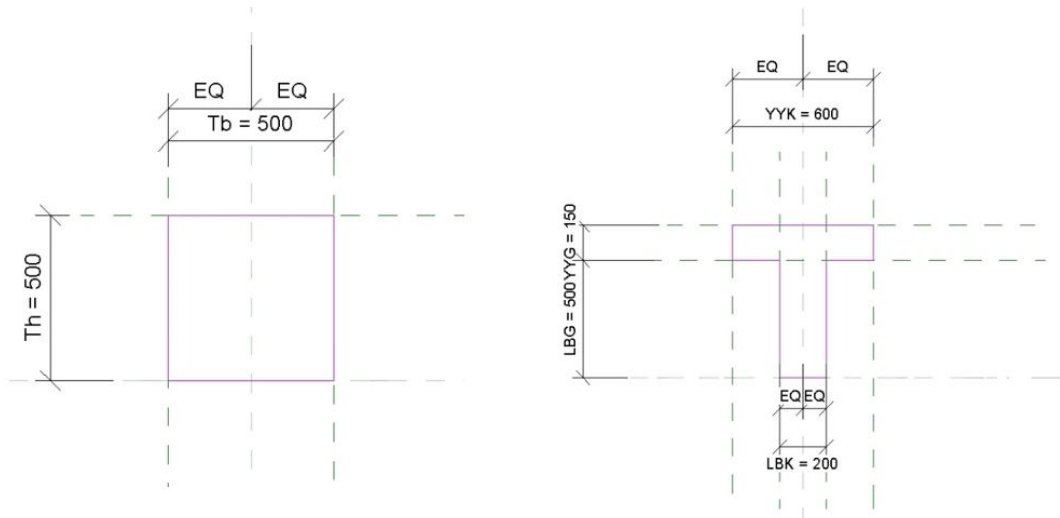
Fig.3. Sections and parameters of tie beam and T-beam
