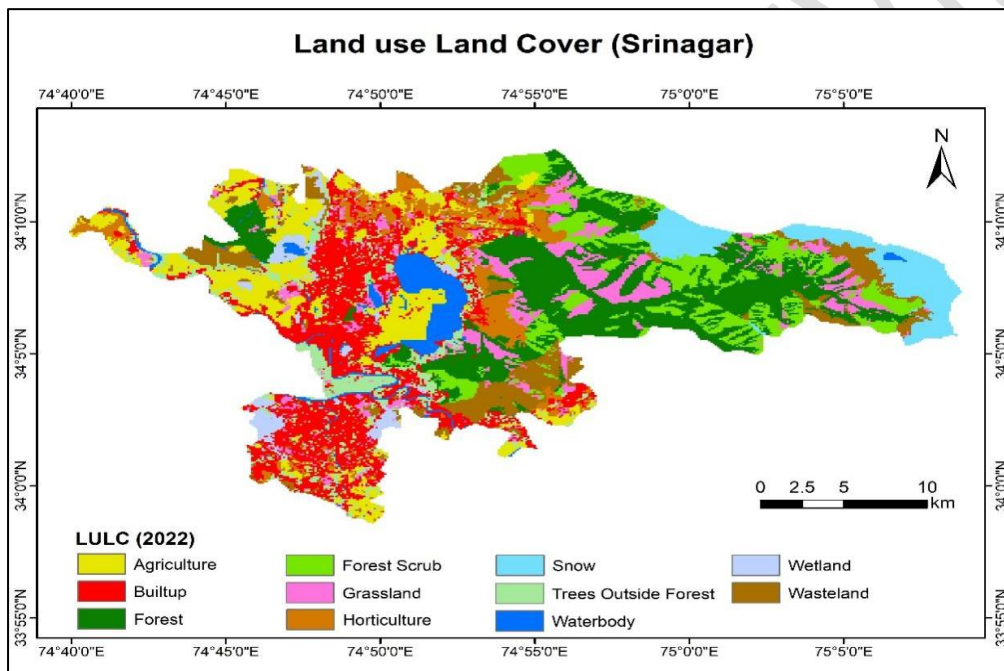
Fig.1: LULC map (2022) of district Srinagar
